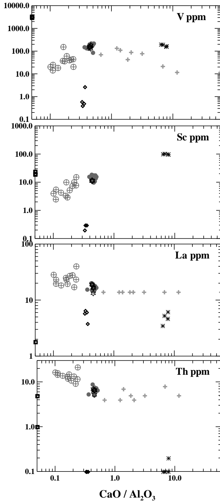
Figure 3. The major (wt%) and trace element contents (ppm) versus CaO/Al 2 O 3 ratio in the 2010 glass inclusions, matrix glasses and phenocrysts compared to the 2010 Merapi bulk volcanic rocks and the 1998 crustal xenoliths. The chemical data on the Merapi were obtained from database of MERAPIDATA, (Borisova et al., 2011). The database summarizes the published and unpublished data of Berthommier (1990), Gertisser and Keller (2003a,b), Debaille et al. (2006), Camus et al., (2006) for the Merapi volcanic products; and Chadwick et al. (2007) for the 1998 Merapi calc-silicate xenoliths. The chemical data on the 2010 Merapi are given in Tables 3 and 4 and in Table S1 of ESM.
