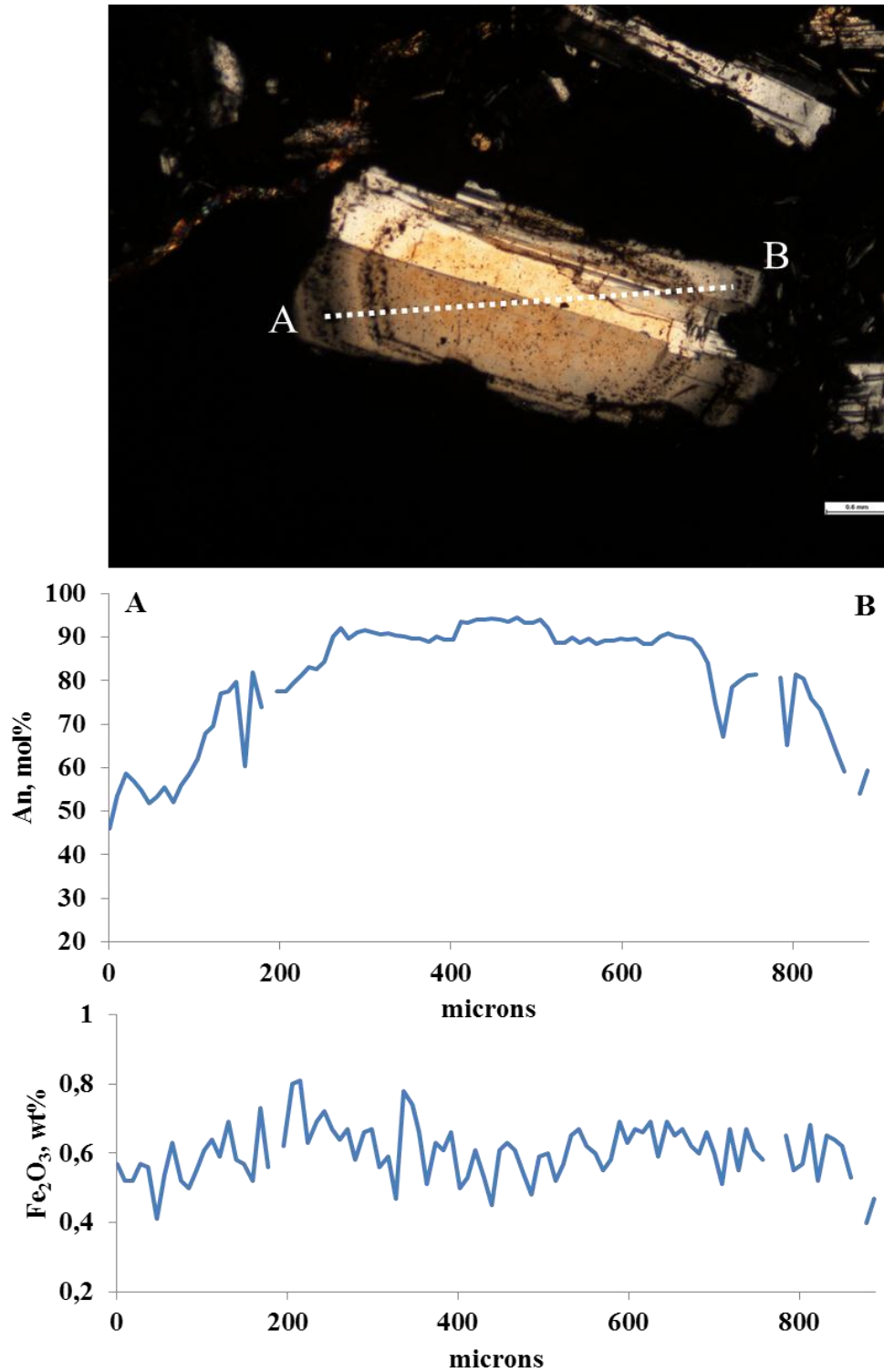
Figure 4 (a). Pyroclastic flow (M 2010 PF) plagioclase phenocryst profiling from A to B points demonstrating extremely enriched in An core ( An_{94} ). The high-An core is chemical signature of assimilation of sedimentary crustal material (see text). Symmetric chemical zonation in An is spectacular. Fe contents demonstrate oscillatory zonation.
