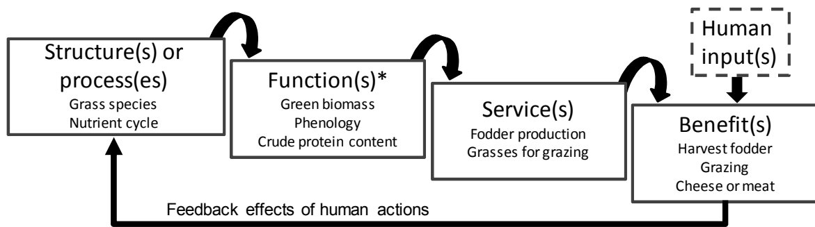
Figure 2: Conceptual cascade of ecosystem services from processes to benefits (adapted from (Haines-Young and Potschin, 2010) and (de Groot et al., 2010)) and example of fodder production in mountain grasslands.
