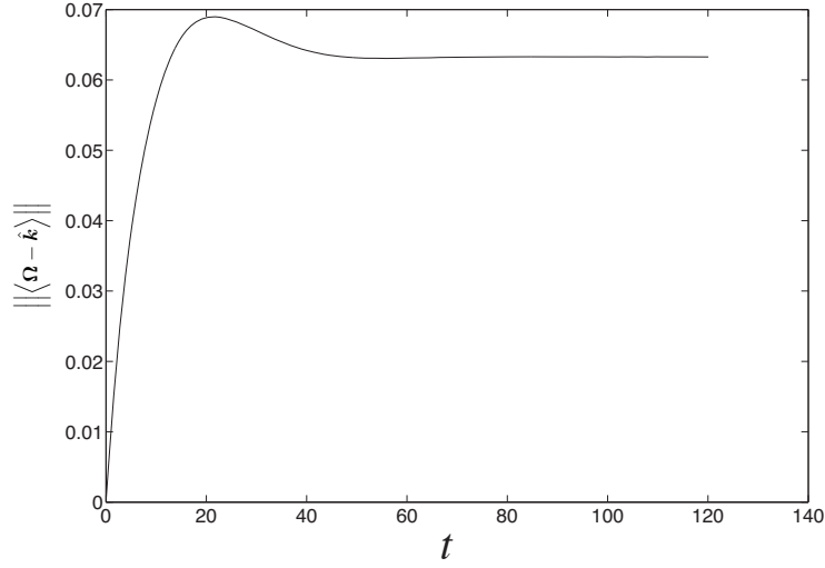
FIGURE 5. Time evolution of the amplitude of the equatorial component of rotation of the fluid in the frame of precession from the simulations. a = b = 1 , c = 0.5 , E = 10^{-3} , Ro = 10^{-2} and Po = -0.45 .
