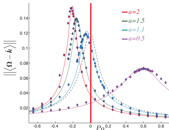
FIGURE 10. Amplitude of the mean differential rotation, \|\langle \boldsymbol{\Omega} - \hat{\mathbf{k}} \rangle\| , as a function of the Poincaré number. The symbols represent numerical simulations at E = 10^{-3} and Ro = 10^{-2} , the solid lines represent the inverted reduced model, the black-dashed line represents the solution for the sphere from Busse (1968). Each geometry, characterized by a , is represented with a different color as indicated. The red vertical line symbolized the region of the parameter space |Po| < 10^{-2} where no \alpha can satisfy Ro = Po \sin(\alpha) .
