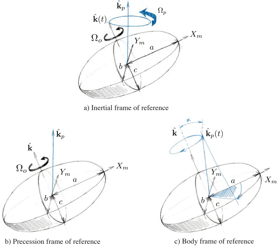
FIGURE 1. Schematic representation of the precessing ellipsoidal cavity. a) As seen from the frame of inertia, b) as seen from the frame of precession and c) as seen from the body frame
