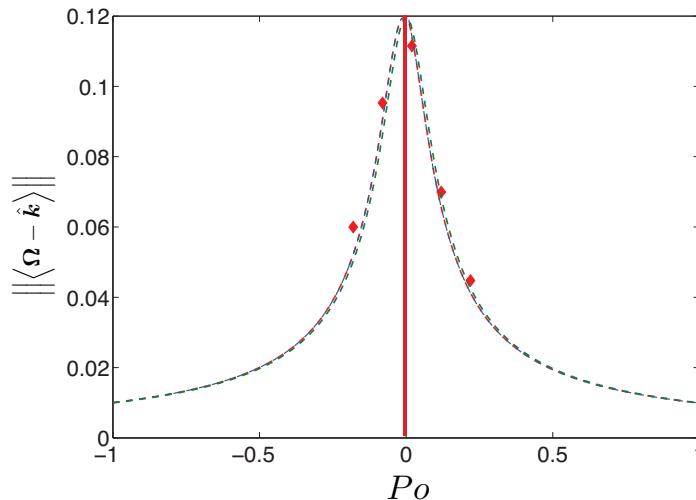
FIGURE 4. Equatorial component of the fluid mean rotation as a function of the Poincaré number in a spherical geometry. The numerical simulations are performed with E = 10^{-3} and Ro = 10^{-2} . The red symbols represent the simulations, the red dashed line represents the asymptotic solution of Busse (1968), the blue dashed line represents the solution of the generalized model (A 14-A 16) and the dashed green line represents the reduced model (2.25-2.27) with a derived value of \lambda = -2.62 . The red vertical line symbolizes the region of the parameter space |Po| < 10^{-2} where no \alpha can satisfy Ro = Po \sin(\alpha) .
