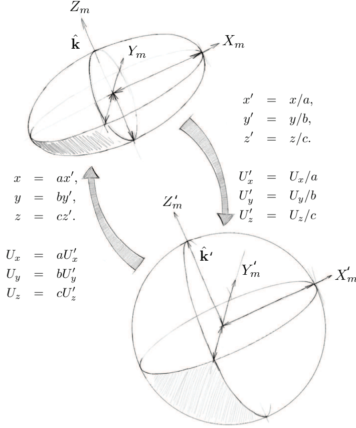
FIGURE 3. Schematic representation of the geometrical stretch that transforms a triaxial ellipsoid into a sphere of radius unity.
