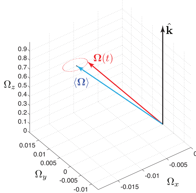
FIGURE 9. Time evolution of the fluid rotation vector \Omega viewed from the frame of precession (Same set of parameters as in Figure 8). The blue arrow represents the mean rotation vector \langle \Omega \rangle , the red arrow represents the instantaneous rotation vector at a particular time, the red dots show the trace of the instantaneous rotation vector for 60 < t < 120 and the black arrow shows the container rotation vector.
