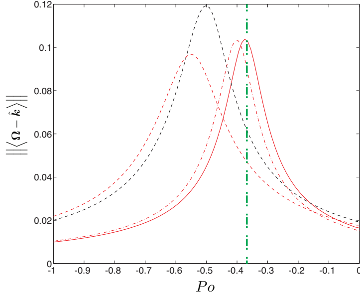
FIGURE 15. Norm of the differential rotation for a = b = 1 , c = 0.5 , E = 10^{-3} , Ro = 10^{-2} . The solid lines represent the reduced models, the dashed line represents the asymptotic theory of Busse (1968); Noir et al. (2003) and the dot-dashed line represents the generalized model. The color scheme stands for the different values of \lambda_{so, i}^r , from Greenspan (1968) (black) and from Zhang et al. (2004) (red). The green dot-dashed line represents the critical Po predicted from a purely inviscid model.
