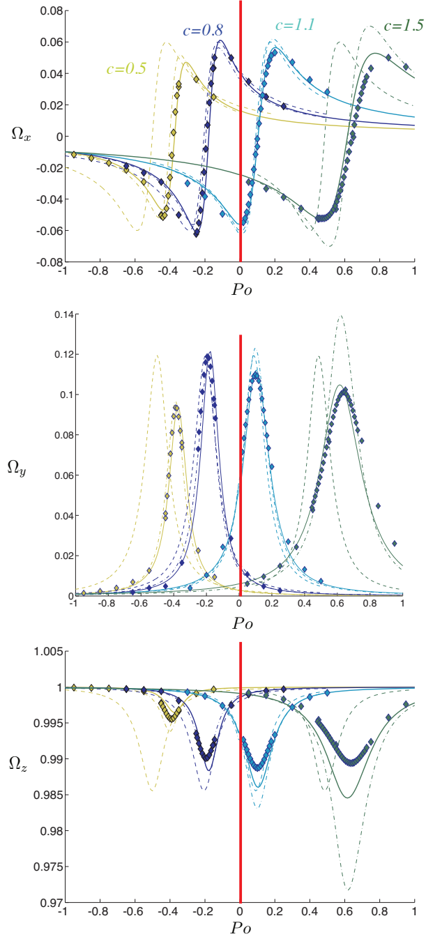
FIGURE 7. From top to bottom: X,Y and Z components of the fluid rotation vector in the frame of precession within an axisymmetric spheroid. We compare our simulations (symbols), the theory of Busse (1968), represented by the dashed lines, our generalization of this model (dot-dashed lines), and the proposed reduced model (solid lines) with the inverted values of \lambda from table 1. Each value of the polar axis c is represented by a different color as indicated. The red vertical line symbolized the region of the parameter space |Po| < 10^{-2} where no \alpha can satisfy Ro = Po \sin(\alpha) .
