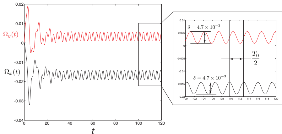
FIGURE 8. Time evolution of the three component of the fluid rotation vector in the frame of precession \Omega_x(t) , \Omega_y(t) from the numerical simulations for a = 0.5 , b = c = 1 , E = 10^{-3} , Ro = 10^{-2} and Po = -0.45 .
