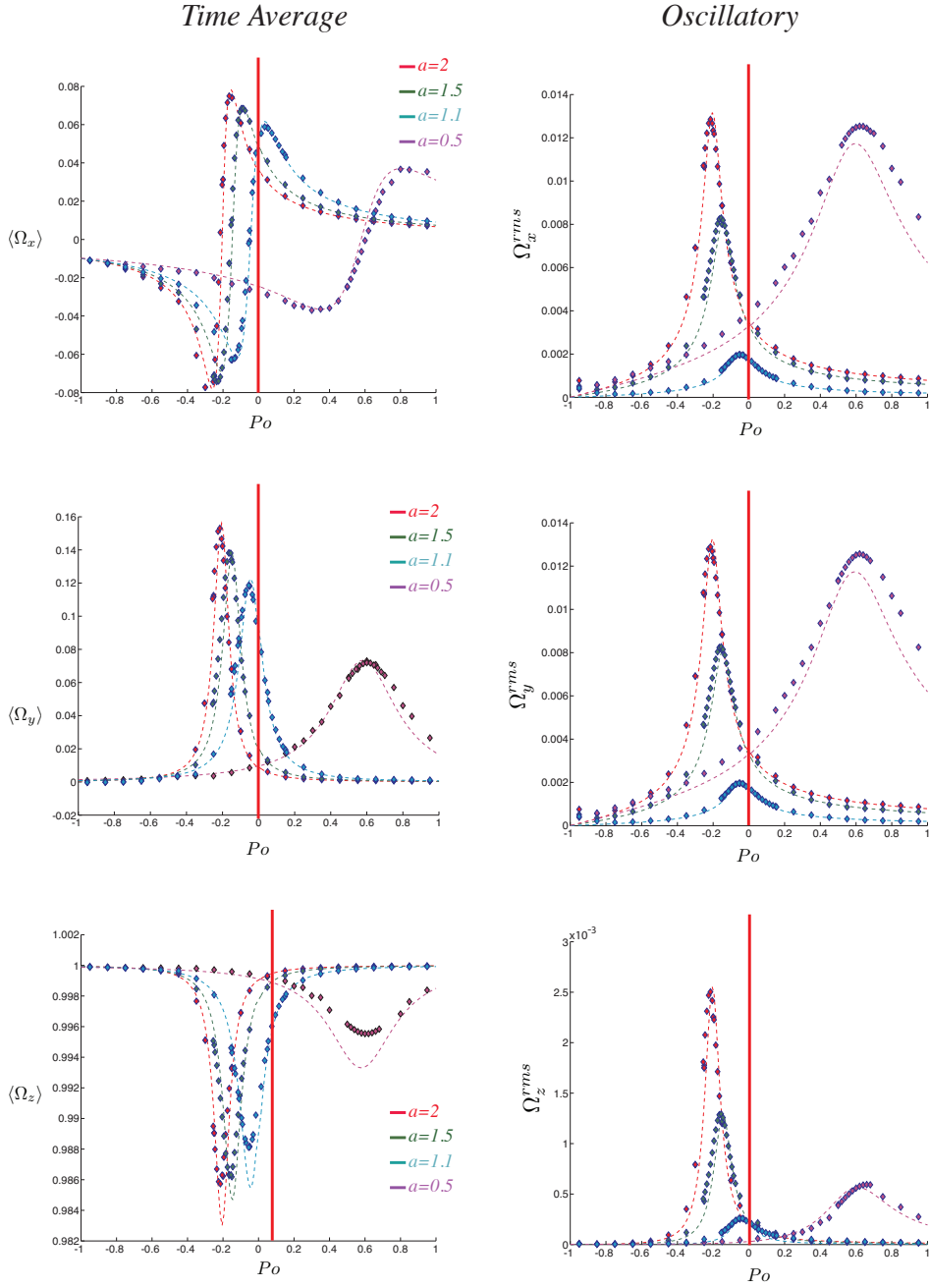
FIGURE 11. From top to bottom: X,Y,Z-component of rotation of the fluid in the frame of precession. The left row shows the time averaged components, the right row shows the time standard deviation of the components. We compare, for each geometry (i.e. a ), our simulations (symbols) and the reduced model (dashed lines) with the inverted values of \lambda from table 2. The red vertical line is the region of the parameter space |Po| < 10^{-2} where no \alpha can satisfy Ro = Po \sin(\alpha) .
