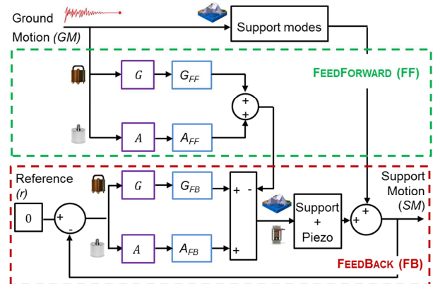
Figure 4: Simplified bloc scheme of the control.
