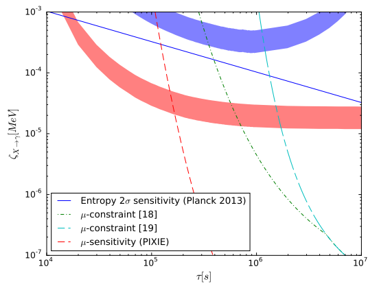
FIG. 1: The lower band is the range of abundance parameter \zeta_{X \rightarrow \gamma} vs. lifetime \tau_X , for which the primordial lithium is depleted to 40% to 70% of its standard value, for a monochromatic photon injection with energy E_0 = 2 \text{ MeV} . The upper band represents the analogous region if we had distributed the same injected energy, up to E_0 = 2 \text{ MeV} , according to the erroneous spectrum of Eq. (1). Above the solid blue curve, a change in entropy (and \Omega_b ) between BBN and CMB time larger than the 2\sigma error inferred from CMB would be obtained. The region to the right of the dot-dashed green curve is excluded by current constraints from \mu -distortions in the CMB spectrum [17] according to the computation of [18], while the dashed cyan curve illustrates the weaker bounds that would follow from the less accurate parameterization of [19]. The dotted red curve is the forecasted sensitivity of the future experiment PIXIE, corresponding to |\mu| \sim 5 \times 10^{-8} [20].
