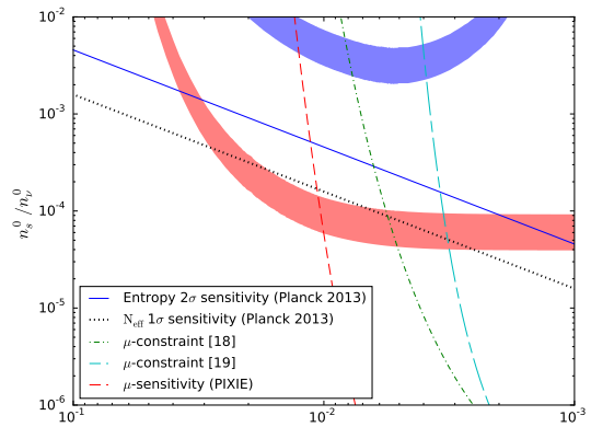
FIG. 2: Constraints for the sterile neutrino model discussed in the text. The legend is the same as for case 1).
