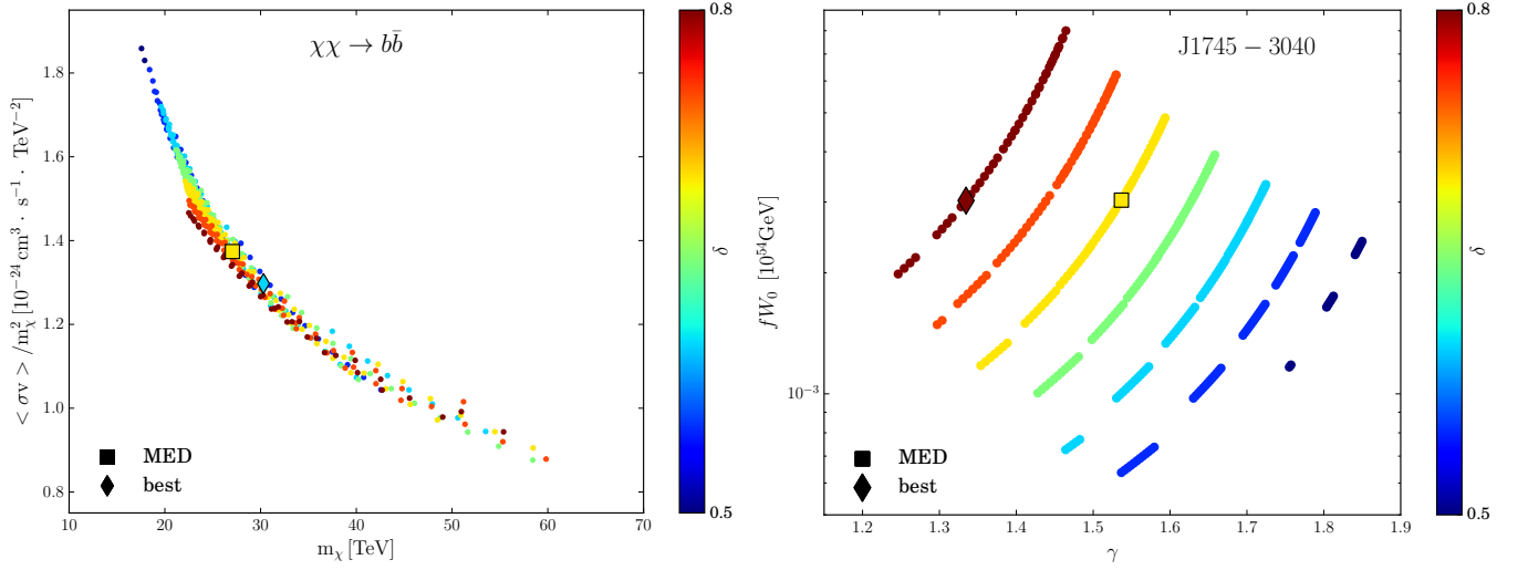
Fig. 16. Surviving transport parameter sets' \delta distributions for the DM \{m_\chi, \langle\sigma v\rangle/m_\chi^2\} (left plot) and the pulsar \{\gamma, fW_0\} (right plot) parameters. The colour coding represents the increasing \delta value from blue to red. The benchmark model MED is represented with a square. In addition, the best transport parameter set is highlighted with a diamond symbol.
