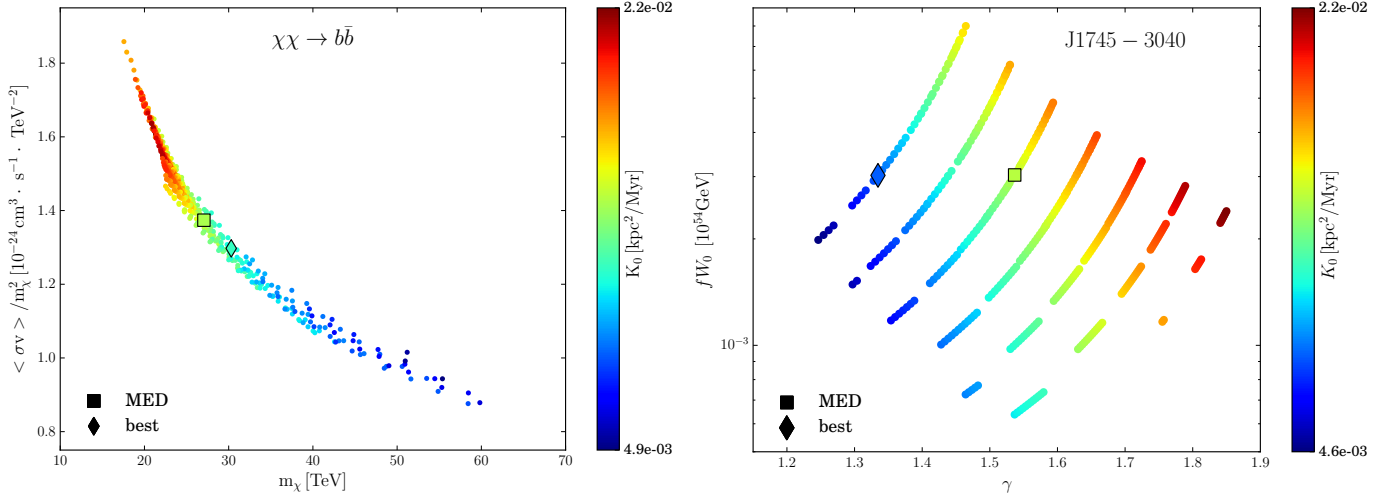
Fig. 15. Surviving transport parameter sets' K_0 distributions for the DM \{m_\chi, \langle\sigma v\rangle/m_\chi^2\} (left plot) and the pulsar \{\gamma, fW_0\} (right plot) parameters. The colour coding represents the increasing K_0 value from blue to red. The benchmark model MED is represented with a square. In addition, the best transport parameter set is highlighted with a diamond symbol.
