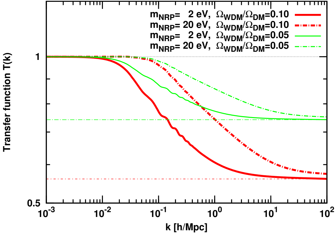
Figure 2: The height of plateau in the transfer function T(k) \equiv [P_{\Lambda\text{CWDM}}(k)/P_{\Lambda\text{CDM}}(k)]^{1/2} depends only on f_{\text{WDM}} only and does not change with the mass. In these examples, the mass is equal to 2 eV (solid line) or 20 eV (dashed-dotted line), while \Omega_{\text{WDM}}/(\Omega_{\text{WDM}}+\Omega_{\text{CDM}}) = 0.1 (red) or 0.05 (green). Other parameters are fixed to \Omega_{\text{B}} = 0.05 , \Omega_{\text{M}} = 0.3 , \Omega_{\Lambda} = 0.7 , h = 0.7 .
