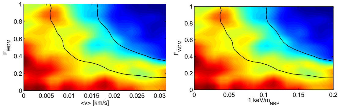
Figure 12: ( Left ) Preferred region for the parameters (F_{\text{WDM}}, \langle v \rangle_{\text{WDM}}) of the \Lambda CWDM model, using SDSS Ly- \alpha and WMAP5 data sets. The black lines represent the 68%CL and 95%CL contours of the two-dimensional probability marginalized over other parameters (as defined in the Bayesian approach), while the colors show the likelihood averaged over other parameters. ( Right ) Same plot with the horizontal axis translated in terms of (1\text{keV}/m_{\text{NRP}}) = \langle v \rangle_{\text{WDM}}/(157\text{ m/s}) , see equation (29).
