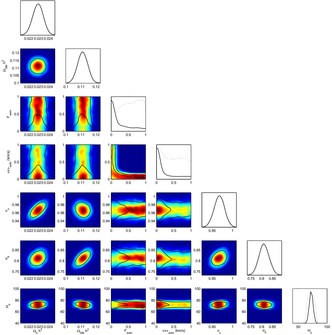
Figure 6: Preferred region for pairs of cosmological parameters in the \Lambda CWDM model, using VHS, WMAP5 and other cosmological data sets. The black lines represent the 68%CL and 95%CL contours of the two-dimensional probability marginalized over other parameters (as defined in the Bayesian approach), while the colors show the likelihood averaged over other parameters. The first five parameters \Omega_B h^2 , \Omega_{\text{DM}} h^2 , F_{\text{WDM}} , \langle v \rangle_{\text{WDM}} , n_s have flat priors over the displayed range. Our analysis also assumes flat priors on the logarithm of the primordial spectrum amplitude and on the angular diameter of the sound horizon, but instead of these parameters we show here \sigma_8 and H_0 , which have a more straightforward interpretation. In this plot, we do not show the reionization optical depth \tau and all the nuisance parameters entering into the analysis. The one-dimensional marginalized probabilities are displayed along the diagonal.
