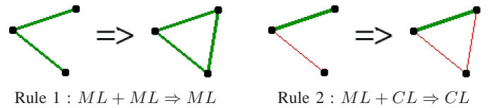
Fig. 2: Constraint propagation.
