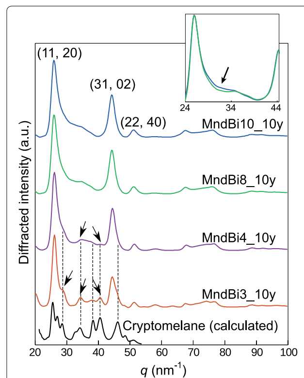
Fig. 1 XRD patterns of the studied samples and of a calculated cryptomelane pattern. Main panel , from top to bottom XRD patterns of MndBi10_10y, MndBi8_10y, MndBi4_10y, MndBi3_10y and a calculated cryptomelane pattern (over the 21–53 \text{nm}^{-1} interval, CSD size of 6 nm). Patterns are scaled for clarity, as maximum intensity diffracted by \delta\text{-MnO}_2 is about 3 % of the maximum intensity diffracted by cryptomelane. Arrows point out to main modulations attributable to a cryptomelane-like structure in MndBi3_10y and MndBi4_10y patterns. MndBi10_10y and MndBi8_10y patterns are overlaid in the inset at the top right to highlight that the hump at 30–33 \text{nm}^{-1} is better defined in MndBi8_10y
