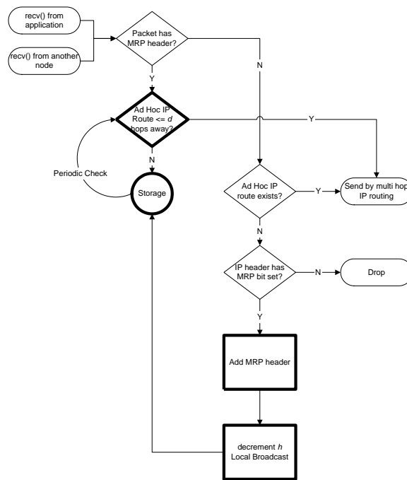
Figure 2: MRP Protocol: Forwarding
