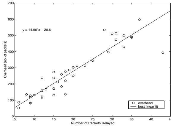
Figure 10: MRP overhead. Each point is the number of broadcasts plus the number of duplicates received over an entire simulation, plotted as a function of the number of relays performed.
