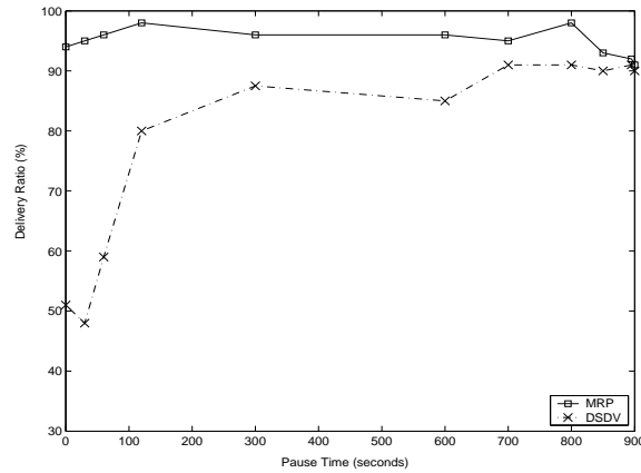
Figure 5: Packet delivery ratio v/s pause time for MRP-enhanced DSDV (MRP) and DSDV on the Soccer Player Model for 50 nodes. before dipping slightly in the completely static case. The behavior observed in our experiments is similar to the one observed in [1] where it is also reported that DSDV fails to converge below pause time 300.
