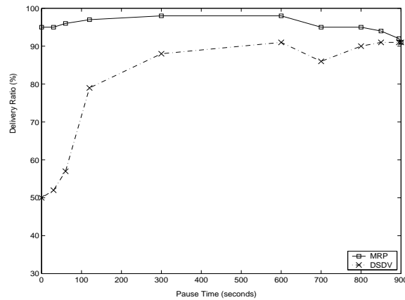
Figure 6: Packet delivery ratio v/s pause time for MRP-enhanced DSDV (MRP) and DSDV on the Homing Pigeon Model for 50 nodes. More interestingly, the performance of MRP on this model is only slightly lower than on the random movement model when pause times are high. This can be explained by the fact that when the pause times are high, the nodes move only once or twice during a simulation. As nodes move mainly in small increments, there is a high probability that a nodes will move relatively slightly during a simulation. Consequently, the overall topology of the network is similar to that of a static network, in which case the performance of MRP is close to the performance of the underlying DSDV. However, overall it is still a noticeable and significant improvement.
