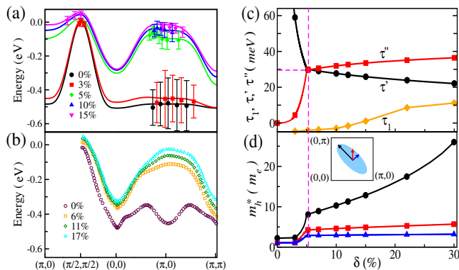
FIG. 1: (Color online) Doping dependent band dispersion obtained from experiment[26, 27] [dots in (a)], Eq.(1) [lines in (a)], and the t - J model[28] (b), with chemical potential at zero. (c) Corresponding \tau , \tau' and \tau'' in the hole picture. (d) Doping dependence of the effective mass of holes m_h^* in the major directions indicated by the arrows in the inset.
