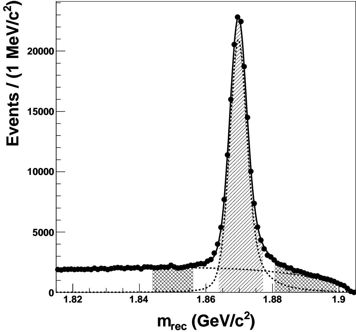
Figure 1. The recoil-mass distribution of K_S^0\pi^+\pi^0 candidates.
