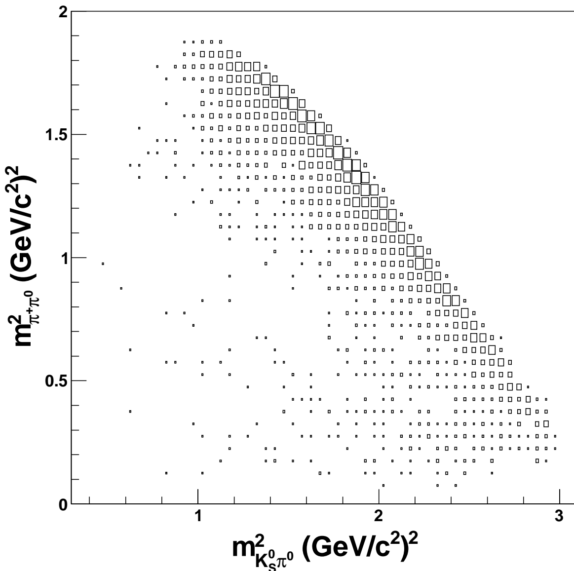
Figure 3. The shape of self-cross-feed events on the Dalitz plot.
