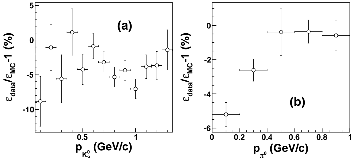
Figure 6. The differences of efficiencies between data and MC as a function of momentum, (a) for K_S^0 and (b) for \pi^0 , for the control samples described in the text.
