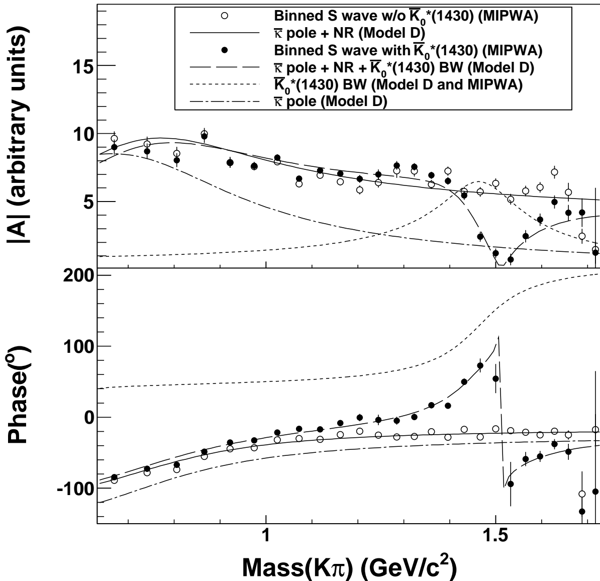
Figure 7. The magnitude and phase of the K\pi S -wave in model D and the MIPWA. The open circles with error bars (statistical uncertainties only) show the binned K\pi S -wave without the K_0^*(1430) and the black dots show the total K\pi S -wave. Other curves show the S -wave components of model D.
