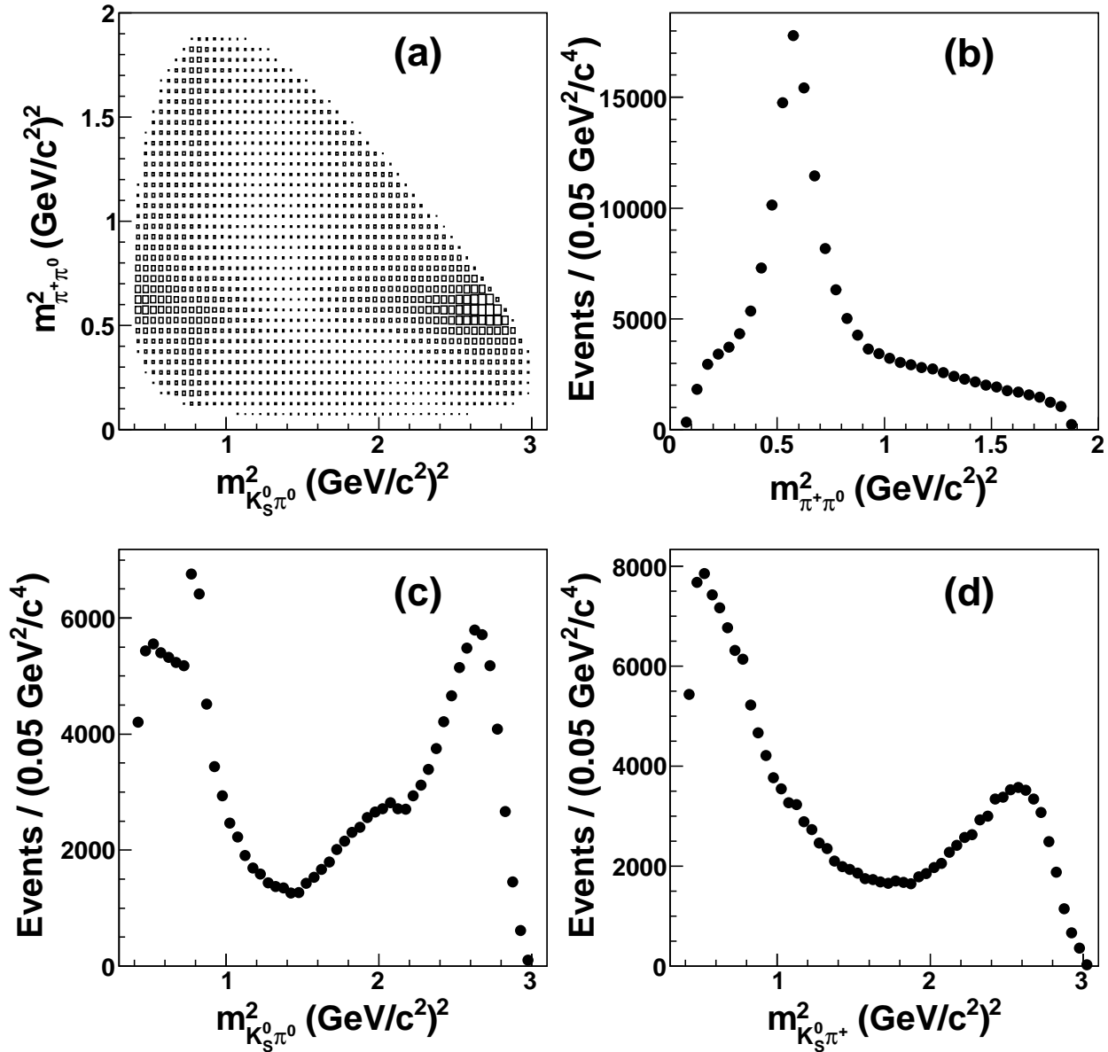
Figure 2. (a) The Dalitz plot for data and the projections onto (b) m_{\pi^+\pi^0}^2 , (c) m_{K_S^0\pi^0}^2 , and (d) m_{K_S^0\pi^+}^2 .
