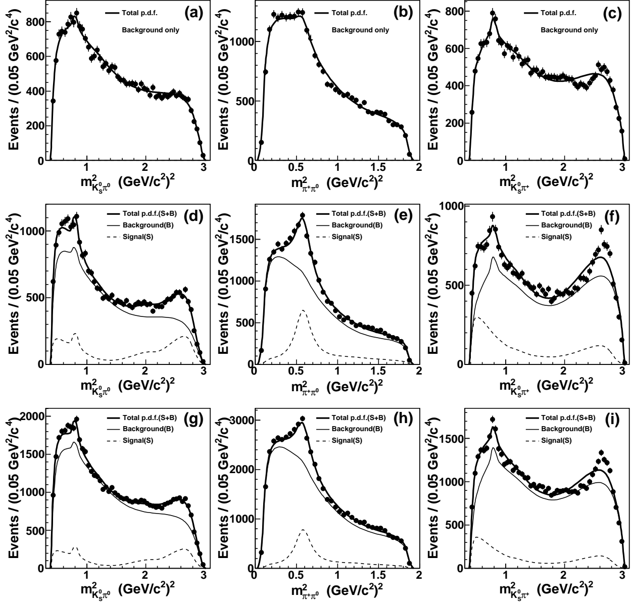
Figure 4. Results of the fit to the sideband backgrounds: (a), (b), and (c) are the three projections for the low-mass sideband only; (d), (e), and (f) are for the high-mass sideband only; and (g), (h), and (i) are for the combined sidebands. The signals are fed in for the signal tail in the sideband of the m_{rec} distribution.
