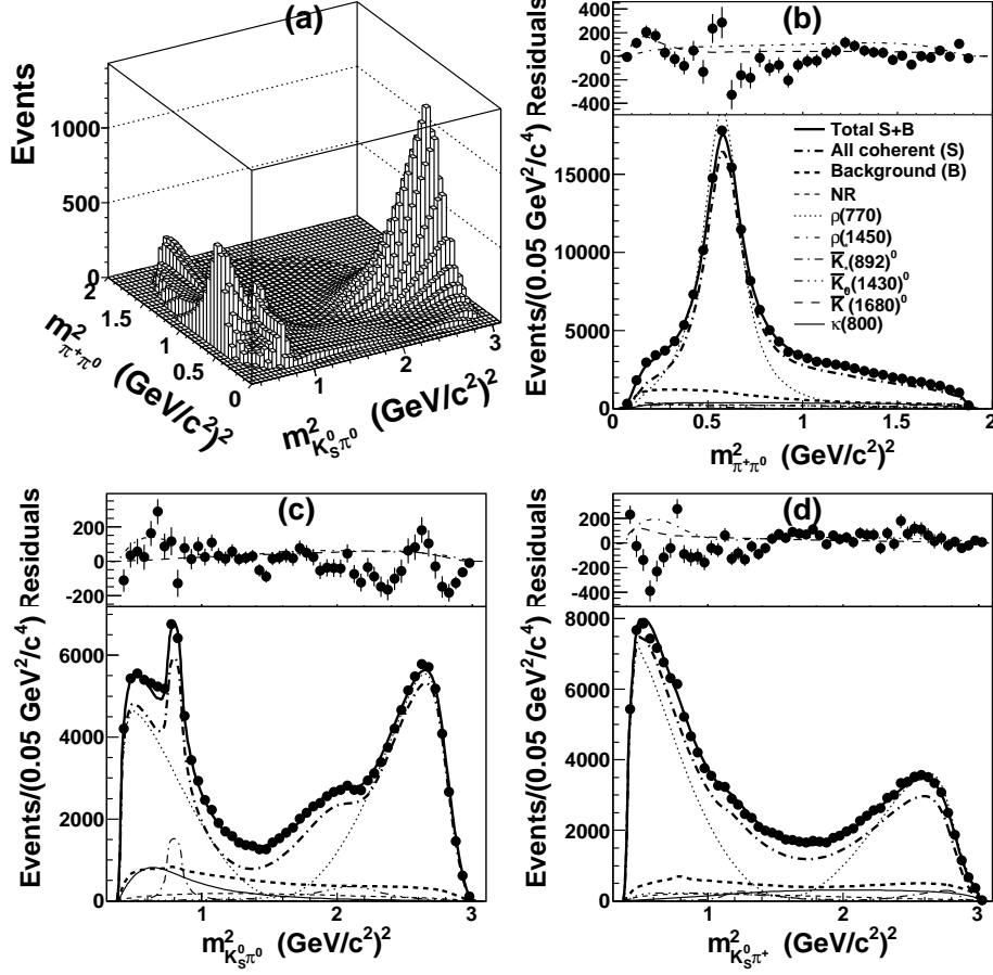
Figure 5. The results of fitting the D^+ \rightarrow K_S^0 \pi^+ \pi^0 data with the model D. (a) Distribution of fitted p.d.f. and projections on (b) m_{\pi^+ \pi^0}^2 , (c) m_{K_S^0 \pi^0}^2 , and (d) m_{K_S^0 \pi^+}^2 . Residuals between the data and the total p.d.f. are shown by dots with statistical error bars in the top insets with minor contributions from the \rho(1450) and the \bar{K}^*(1680)^0 .
