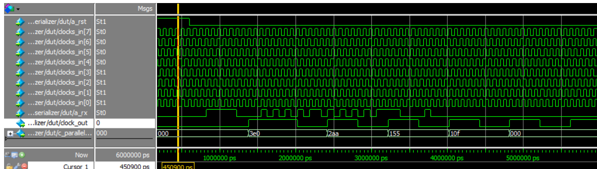
Figure 12. RTL simulation of Deserializer inputs and outputs
