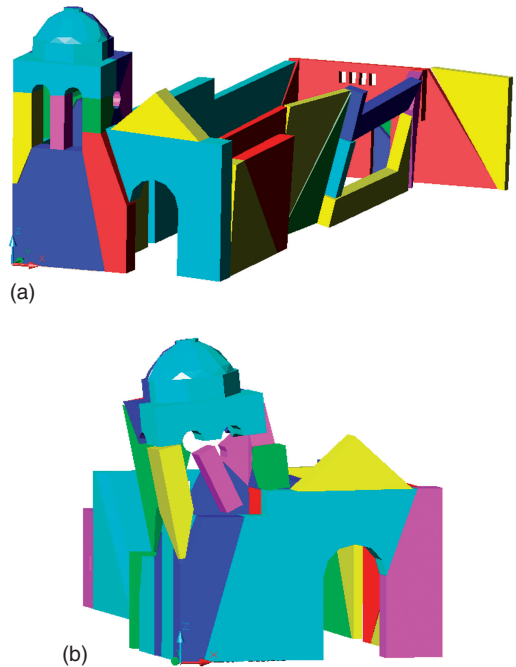
Figure 3. Case 1 failure mechanisms for seismic action on (a) +X direction; and (b) -X direction.
