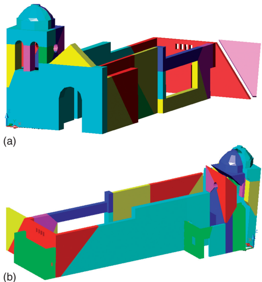
Figure 4. Case 1 failure mechanisms for seismic actions on (a) +Y direction; and (b) -Y direction.
