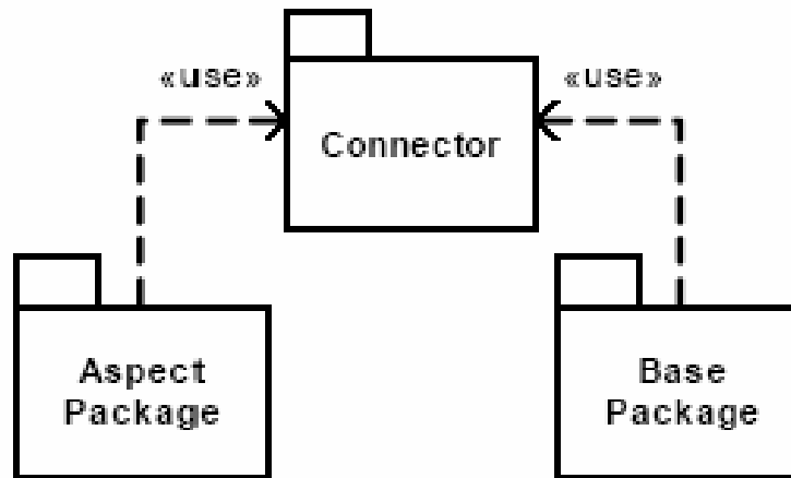
Figura 17. AML aspect, connector and base Fuente: [8]
