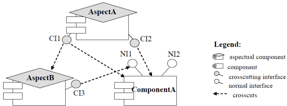
Figura 11. Architectural aspects and crosscutting interfaces
