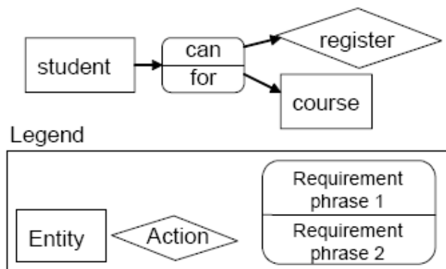
Figura 3 Theme View from Theme/Doc Tool for a course of Registration System
