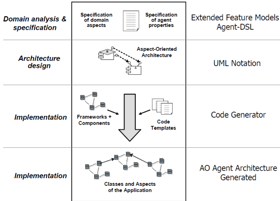
Figura 9. The development phases covered by the AOGA approach Fuente: [2]
