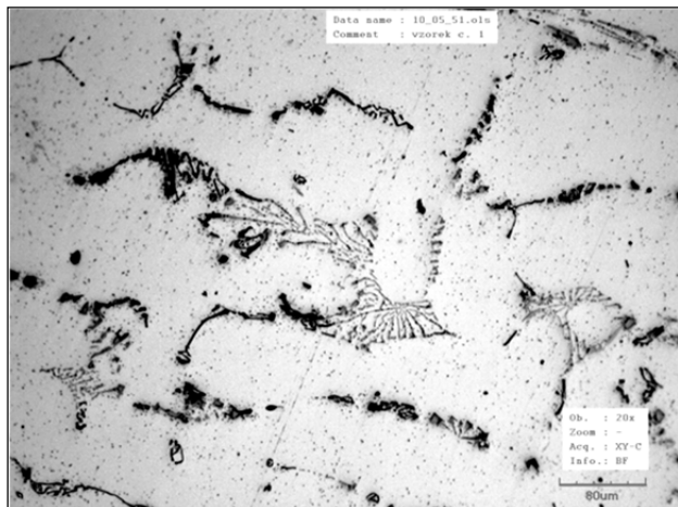
Fig. 8. Microstructure of Cast No. 2
