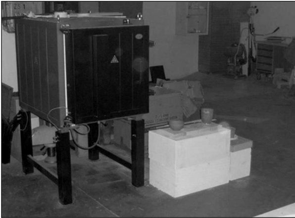
Fig. 5. Electrical Resistance Furnace LAC
