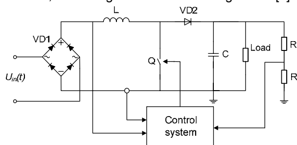
Fig. 1. Power factor corrector based on a boost converter
