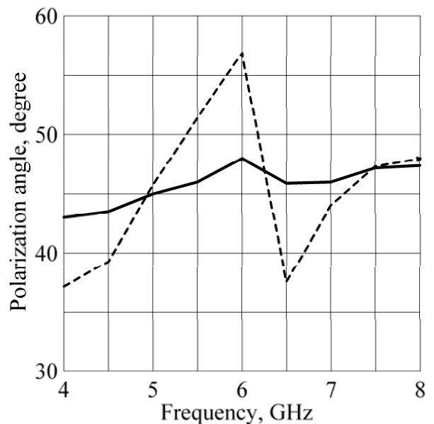
Fig.10. Polarization tilt angle of 16-element subarray: case of standalone subarray (solid line); case of two closely disposed subarrays with horns rotated to -45^\circ and +45^\circ (dashed line).
