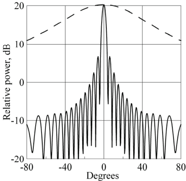
Fig. 5. Calculated radiation pattern of 16-element horn array with linear polarization angle 45^\circ at frequency 6 GHz: vertical plane (solid line); horizontal plane (dashed line).
