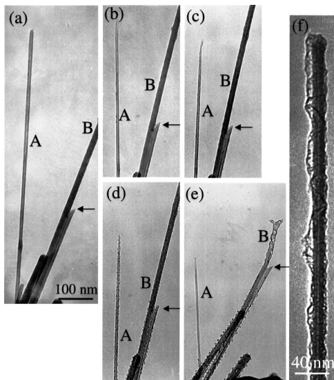
FIG. 4. “Stripping” effect in structural damage. (a)–(e) Series of TEM images showing the structural damage of a carbon nanotube during field emission. The applied voltages were (a) V=100 V, (b) V=120 V, (c) V=140 V, (d) V=160 V, and (e) V=200 V. The distance from the tip of the nanotube to the counterelectrode was \sim 4 \mu\text{m} . (f) A carbon nanotube after passing through a large current, showing the structural damage at the outer graphitic layers, while the internal layers are intact.
