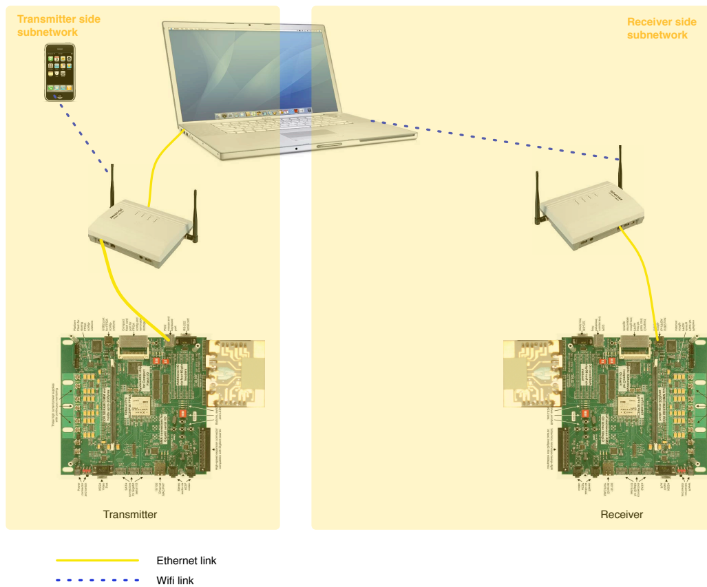
Figure 16: Network setup
