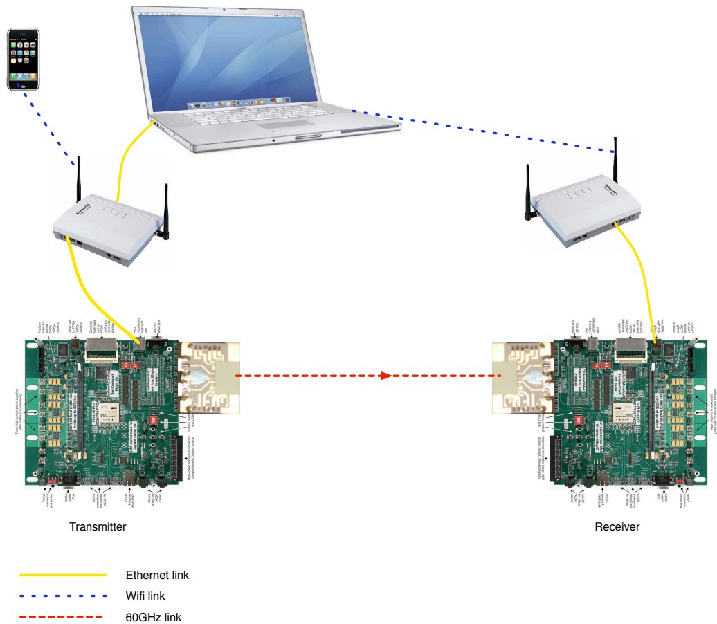
Figure 1: Schematic view of the demonstration setup
