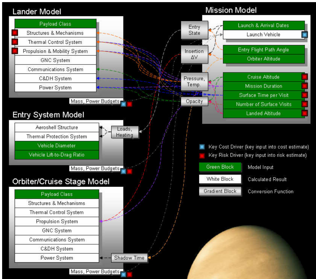
Figure 14. Notional VISE Vehicle and Mission Modeling Framework.
