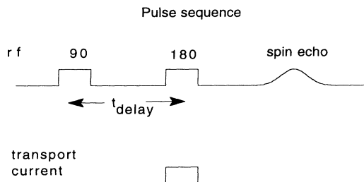
FIG. 3. The timing diagram for pulse sequences containing pulses of transport current. The transport current is pulsed on during the 180^\circ RF pulse. For a static vortex lattice, current pulses exceeding the critical current density will displace the vortex lattice and rephasing after the 180^\circ pulse should be diminished. For all current pulses investigated the spin-echo size is unaffected.
