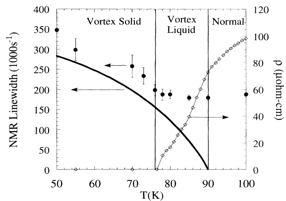
FIG. 1. Resistivity and ^{63}\text{Cu} NMR linewidth as a function of temperature for the twinned YBCO crystal in a 9 T field applied parallel to the crystalline c axis. No broadening of the ^{63}\text{Cu} line shape is seen down to temperatures below which the resistance becomes effectively zero.
