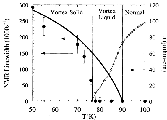
FIG. 2. Resistivity and vortex lattice contribution to the second moment of the ^{63}\text{Cu} NMR line shape as a function of temperature. The 9 T applied field is parallel with the crystal-line c axis. The solid line is the prediction based on a static vortex lattice using the penetration depth values from Hardy et al. and Eq. (1).
