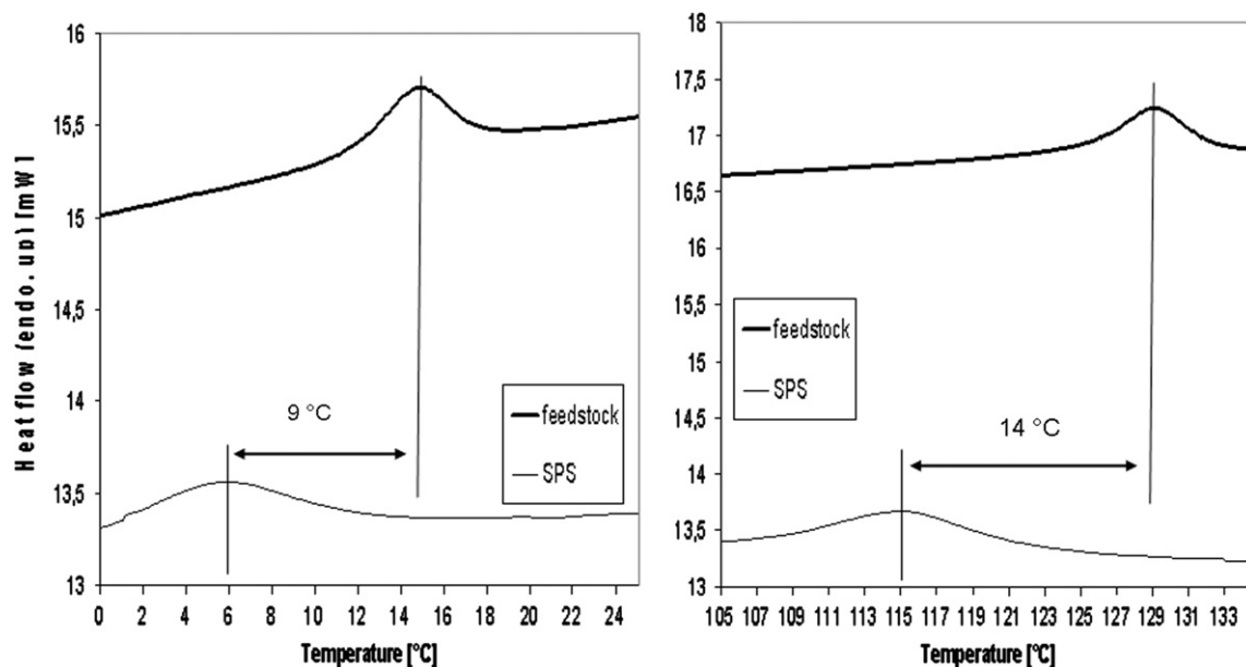
Fig. 9. Details of the DSC curves of the feedstock and SPS bulk around the transformation temperatures.
