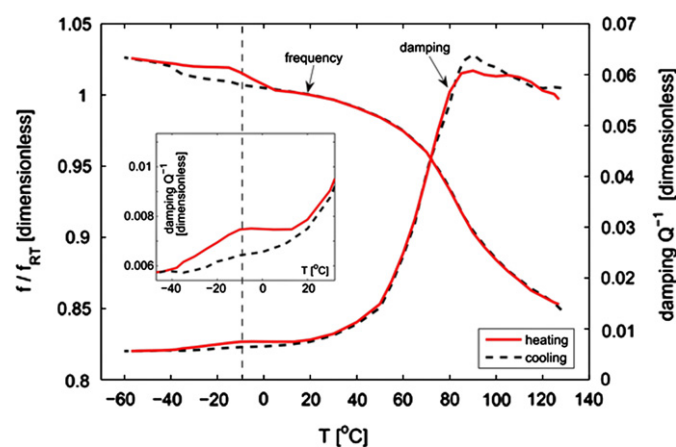
Fig. 3. Temperature dependence of the frequency of the chosen mode from the RUS spectrum (left vertical axis) and of the corresponding damping (right vertical axis) for the GSP coating. The zoomed area shows the damping peak corresponding to the reverse structural transition in low temperatures.
