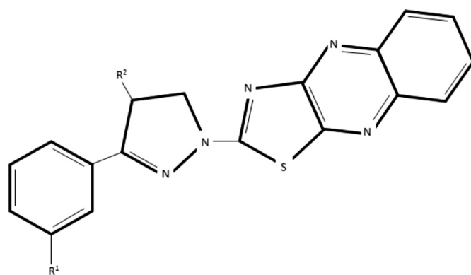
Fig. 7. 1-[Thiazolo[4,5-b]quinoxaline-2-yl]-3-phenyl-2-pyrazolines core.
