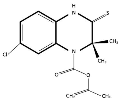
Fig. 5. 6-Chloro-3,3-dimethyl-4-(isopropenyloxycarbonyl)-3,4-dihydroquinoxalin-2(1H)-thione.
