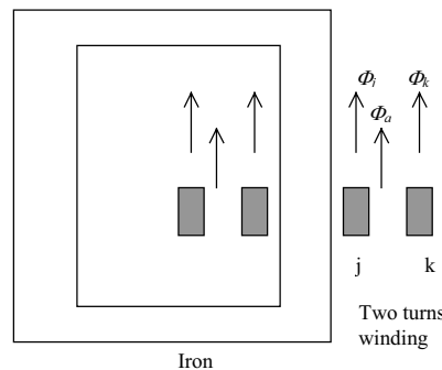
Figure 5: Transformer with a two-turn winding
