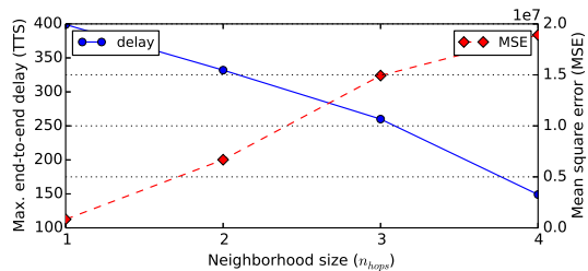
Fig. 7: Trade-off between mean square error and maximum end-to-end delay for different values of n_{hops} .
