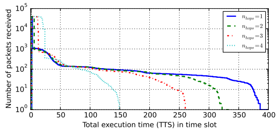
Fig. 8: Number of receptions over time for different values of n_{hops} .
