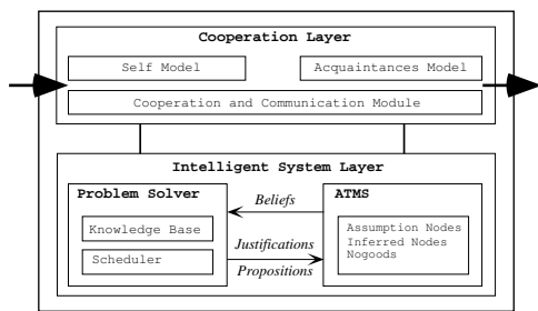
Figure 1: Agent Architecture
