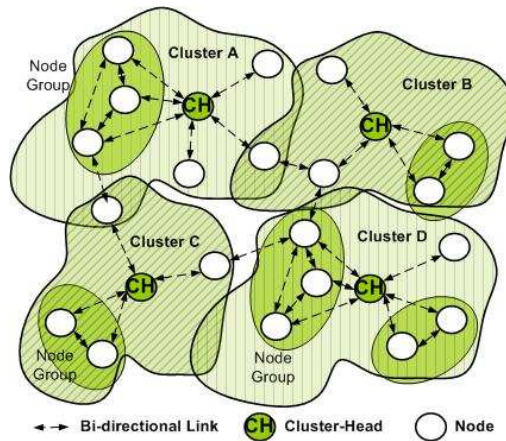
Fig. 3 : Network model
