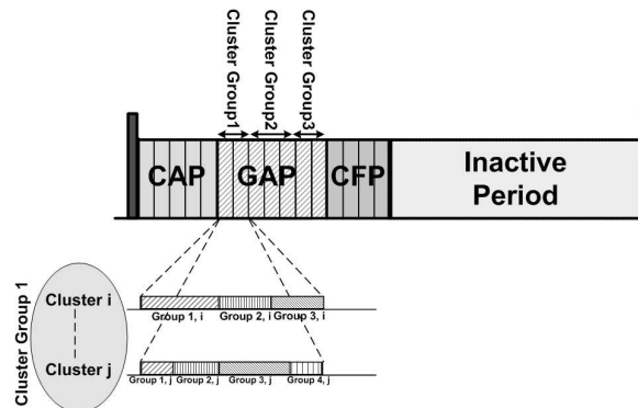
Fig. 16. Medium access mechanism with H-NAME approach
