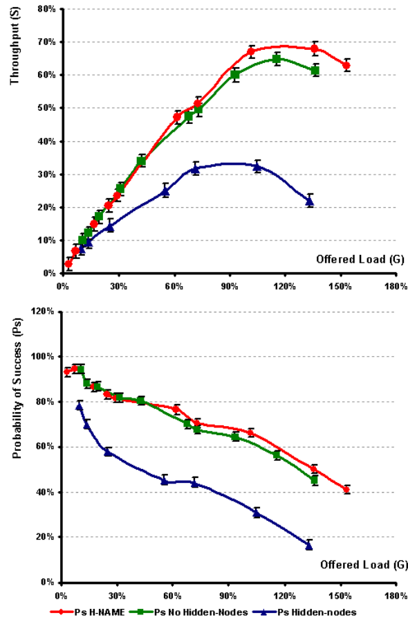
Fig. 20. Experimental performance results
