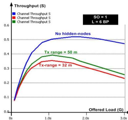
Fig. 2: Hidden-node impact on network throughput
