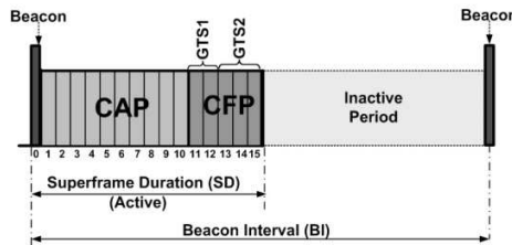
Fig. 8. Superframe structure
