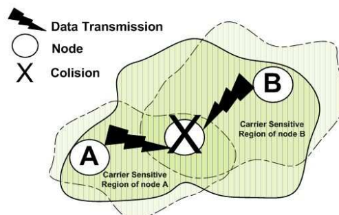
Fig. 1: A hidden-node collision
