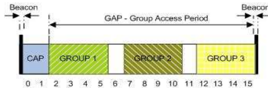
Fig. 18. Groups allocation in the superframe
