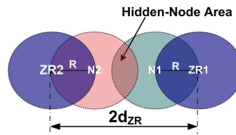
Fig. 13. Hidden-Node Area
