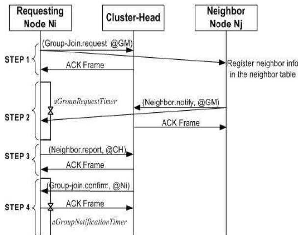
Fig. 5: Intra-cluster grouping message sequence chart
