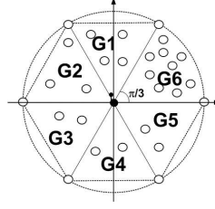
Fig. 6. Maximum number of group in a cluster assuming bi-directional links and circular radio range
