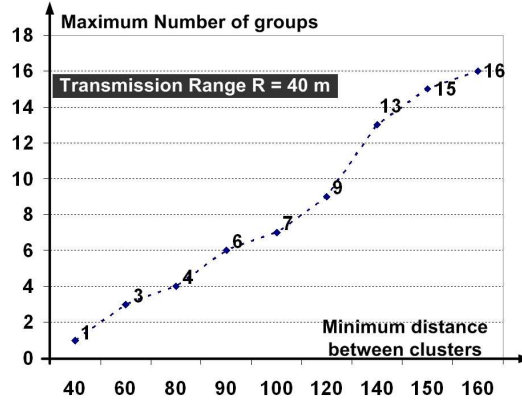
Fig. 12. Relation between maximum number of groups and minimum distance between clusters
