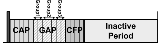
Fig. 9. CAP, GAP and CFP in the Superframe
