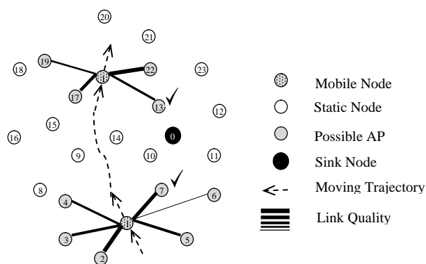
Figure 1 – Network scenario
