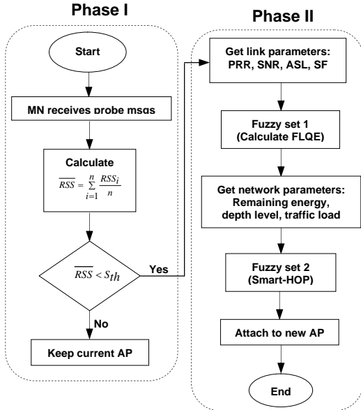
Figure 2— smart-HOP algorithm (simplified)
