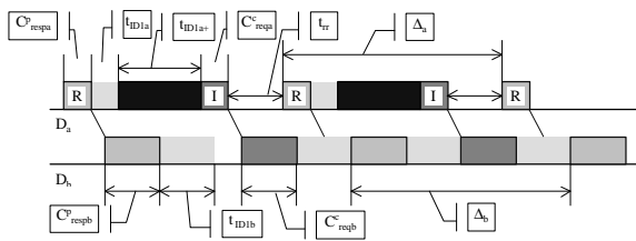
Figure 2: Inserting additional idle time (acknowledged request sequence)
