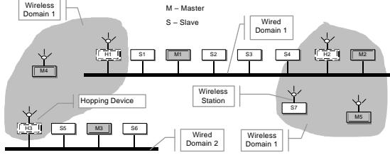
Figure 4: RFieldbus network topology and components
