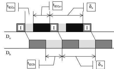
Figure 3: Inserting additional idle time (unacknowledged request sequence)
