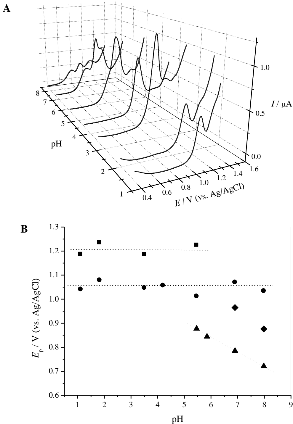
Figure 1. A) 3D plot and B) plots of E_p (filled symbols) and I_p (open symbols) vs. pH from DP voltammograms of 0.1 mM solutions of tamoxifen in different buffer electrolytes as a function of pH. (●) first peak, (■) second peak; (▲) third peak and (◆) fourth peak (error bars are constructed for five measurements). Scan rate 5 \text{ mV s}^{-1} .
