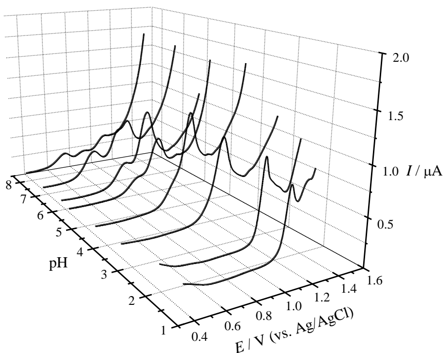
Figure 2. 3D plot from DP voltammograms of 0.1 mM solutions of ( E )-tamoxifen in different buffer electrolytes as a function of pH. Scan rate 5 \text{ mV s}^{-1} .
