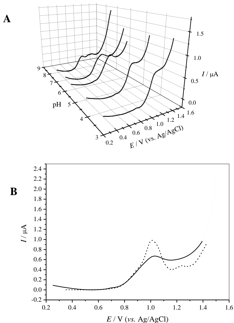
Figure 3. A) 3D plot from DP voltammograms of 0.1 mM solutions of dihydrotamoxifen in different buffer electrolytes as a function of pH. Scan rate 5 \text{mV s}^{-1} . B) DP voltammograms of 0.1 mM solutions of (—) dihydrotamoxifen, (---) tamoxifen and (•••) N -Desmethyl tamoxifen in pH 5 buffer electrolyte. Scan rate 5 \text{mV s}^{-1} .
