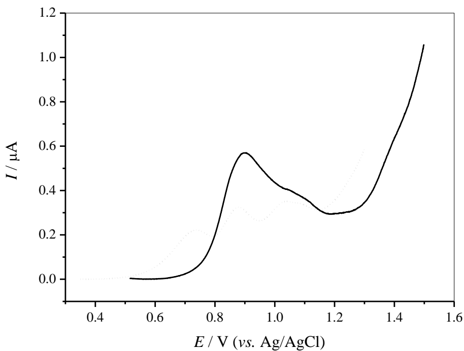
Figure 6. DP voltammograms of 0.1 mM solutions of (—) N -Desmethyl tamoxifen and (•••) tamoxifen in pH 7 buffer electrolyte. Scan rate 5 \text{ mV s}^{-1} .
