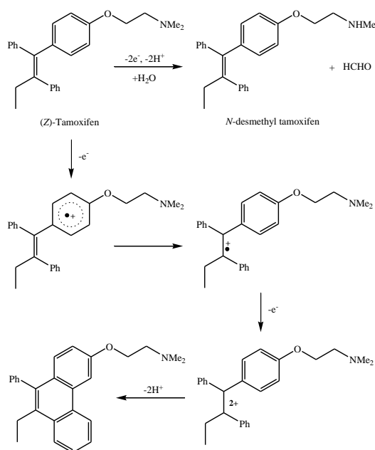
Scheme 2. Proposed mechanism for the electrochemical oxidation of tamoxifen.
