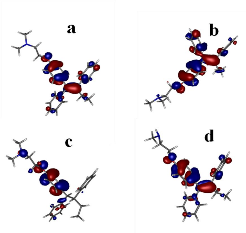
Figure 4. Representation of the Highest Occupied Molecular Orbital (HOMO) for a) tamoxifen, b) ( E )-tamoxifen, c) dihydrotamoxifen and d) N -Desmethyl tamoxifen. Determined at the B3LYP/6-31++G** level of theory.
