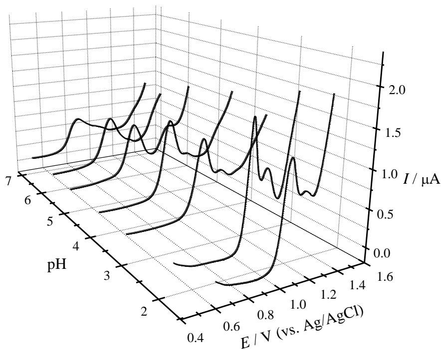
Figure 5. 3D plot from DP voltammograms of 0.1 mM solutions of N -Desmethyl tamoxifen in different buffer electrolytes as a function of pH. Scan rate 5 \text{ mV s}^{-1} .
