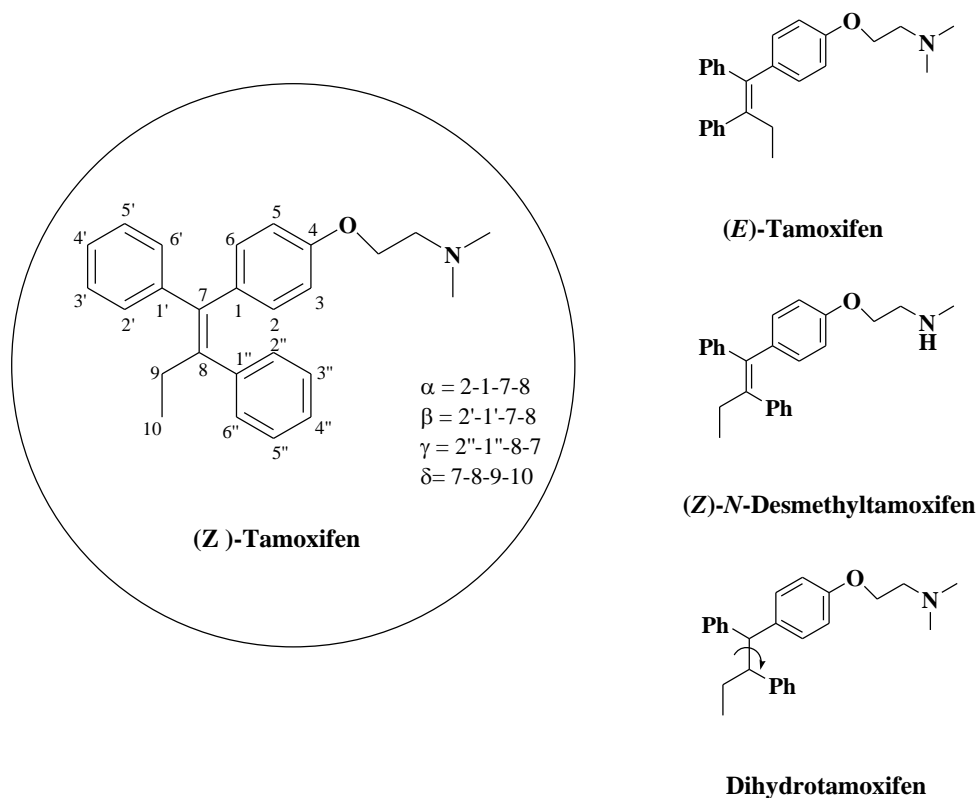
Scheme 1. Chemical structures of tamoxifen, ( E )-tamoxifen, dihydrotamoxifen and N -desmethyl tamoxifen.
