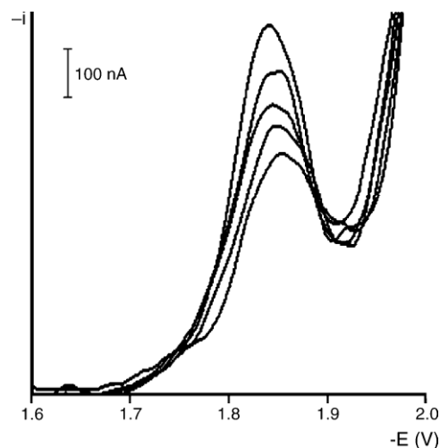
Fig. 5. Typical flow injection voltammograms obtained in the quantification of STR in a pharmaceutical preparation (Zoloft) using the standard addition method. Standard additions of STR ( 10^{-7} \text{ mol L}^{-1} ): 0, 3.00, 4.00, 5.00 and 6.00. E_{\text{acc}} : -1.2 \text{ V} , t_{\text{acc}} : 15 s, f : 10 Hz, E_{\text{step}} : 5 mV, E_{\text{amp}} : 25 mV and flow rate: 1.1 \text{ mL min}^{-1} .
