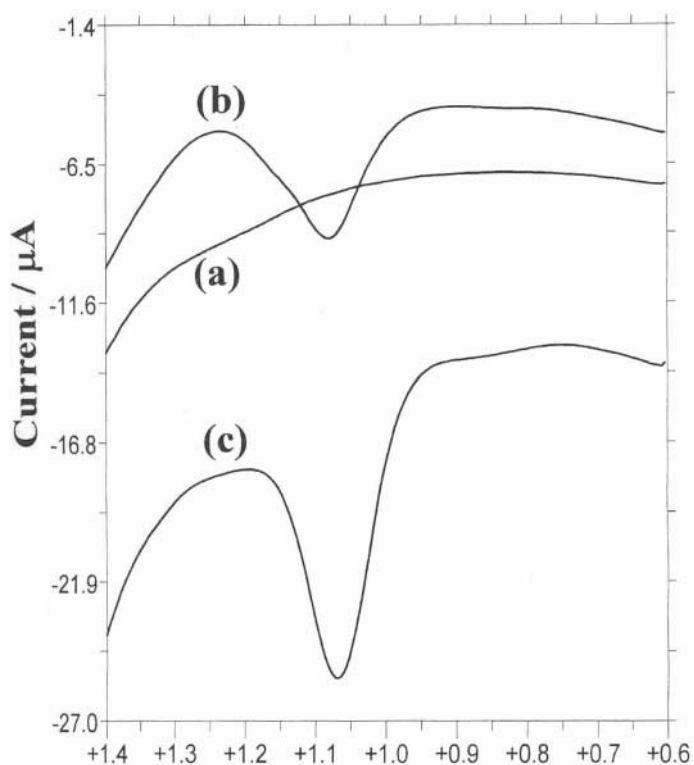
Figure 5. SW voltammograms for 10 \mu\text{M} codeine in 0.05 M \text{HClO}_4 solution at a bare GCE (a), the Nafion/GCE (b), and the Nafion/ruthenium oxide pyrochlore chemically modified electrode (c). SWV amplitude: 50 mV; SW frequency: 15 Hz; step height: 4 mV. Reproduced with permission from Ref. [30] .
