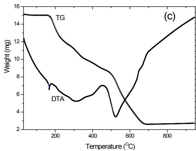
Fig. S-2 TG-DTA plots of 1 (a), 2 (b) and 3 (c)
