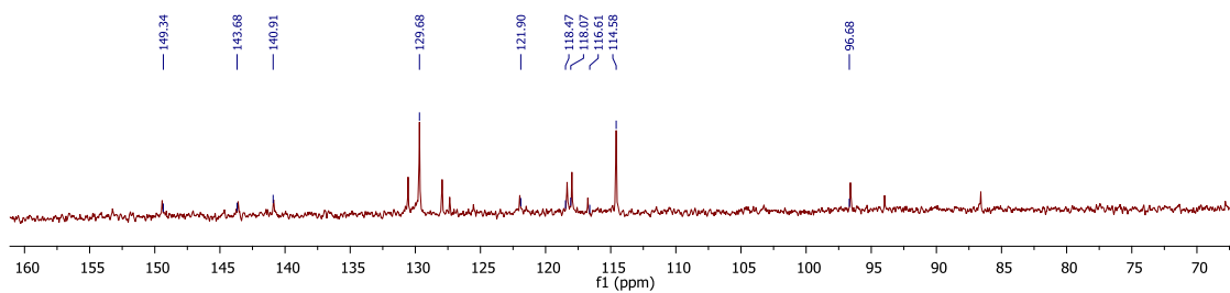
Figure S3.2 - ^{13}\text{C-NMR} spectrum of compound 1 in (\text{CD}_3)_2\text{CO} (400MHz)
