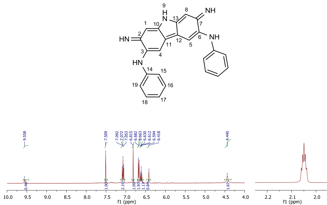
Figure S3.1 - ^1\text{H-NMR} spectrum of compound 1 in (\text{CD}_3)_2\text{CO} (400MHz), with expansion of solvent region
