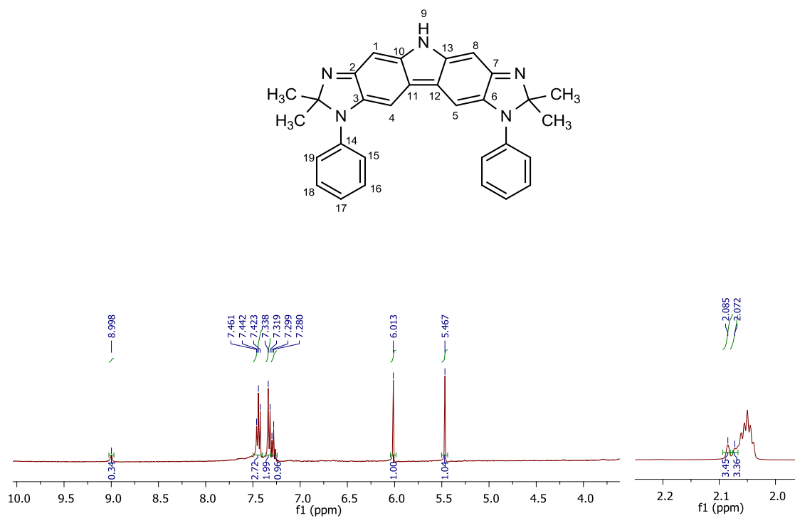
Figure S3.6 - ^1\text{H-NMR} spectrum of compound 2 in (\text{CD}_3)_2\text{CO} (400MHz) with expansion of solvent region
