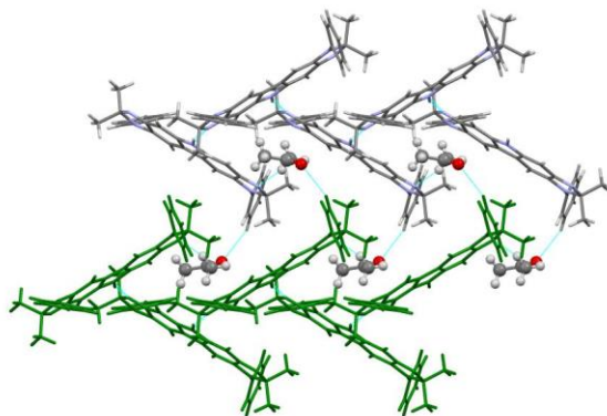
Figure S2.1 – View of three-dimensional packing pattern of compound 2
