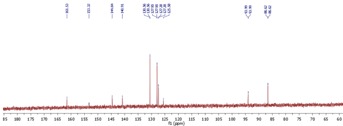
Figure S3.7 - ^{13}\text{C-NMR} spectrum of compound 2 in (\text{CD}_3)_2\text{CO} (400MHz)
