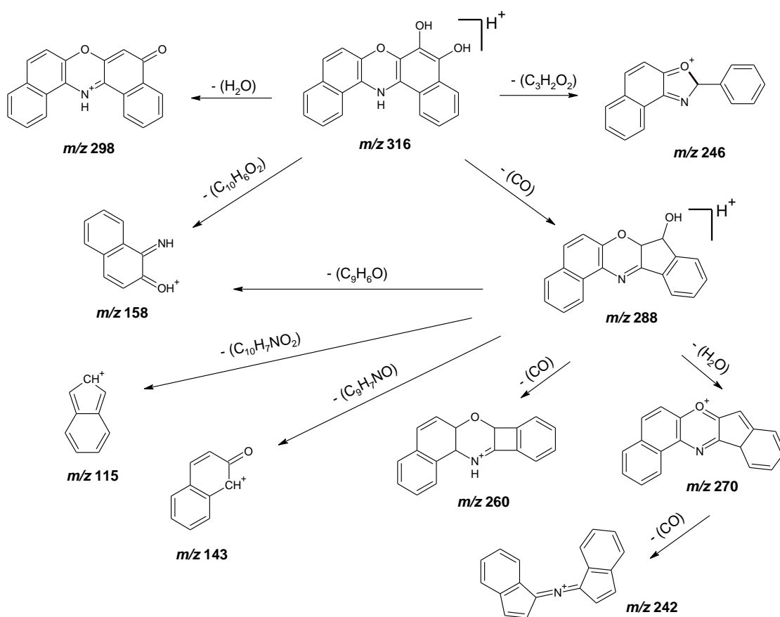
Figure S1 - Proposed fragmentation mechanism of compound 9
