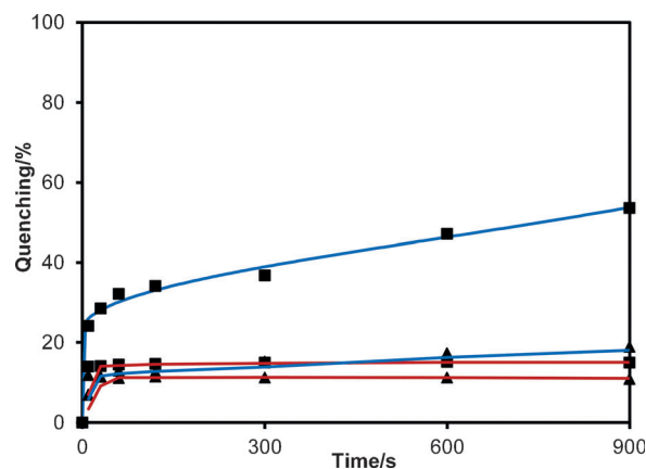
Figure 6. Fluorescence quenching efficiencies for thin films ( \approx 15 and 50 nm, respectively) of TBP-PPE-2,7-CBZ (red) and TBP-PPE-3,6-CBZ (blue) with NM (■) and DMNB (▲), after excitation at \lambda = 360 nm.
