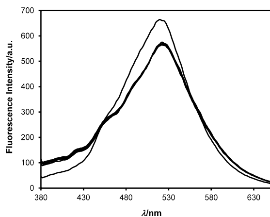
Figure 5. Time-dependent emission intensities of a TBP-PPE-2,7-CBZ thin film ( \approx 15 nm) after being exposed to saturated NM at 25 °C (0, 10, 30, 60, 90, 120, 300, 600, and 900 s, from top to bottom; \lambda_{\text{exc}} = 360 nm).
