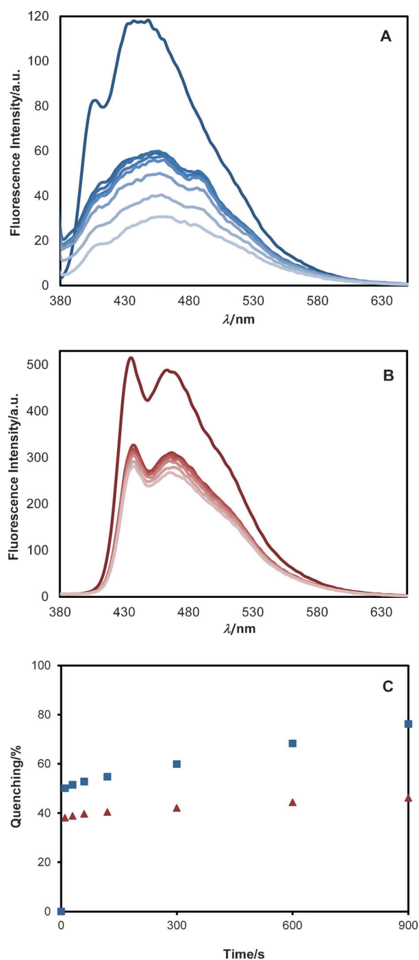
Figure 2. Time-dependent emission intensities of A) CALIX-PPE-3,6-CBZ and B) CALIX-PPE-2,7-CBZ thin films ( \approx 20 nm) after being exposed to saturated NM vapor (47270 ppm) at 25 °C (0, 10, 30, 60, 90, 120, 300, 600, and 900 s, from top to bottom), and the corresponding fluorescence quenching efficiencies (C) for both materials ( \blacksquare from A, \blacktriangle from B; \lambda_{\text{exc}} = 360 nm).
