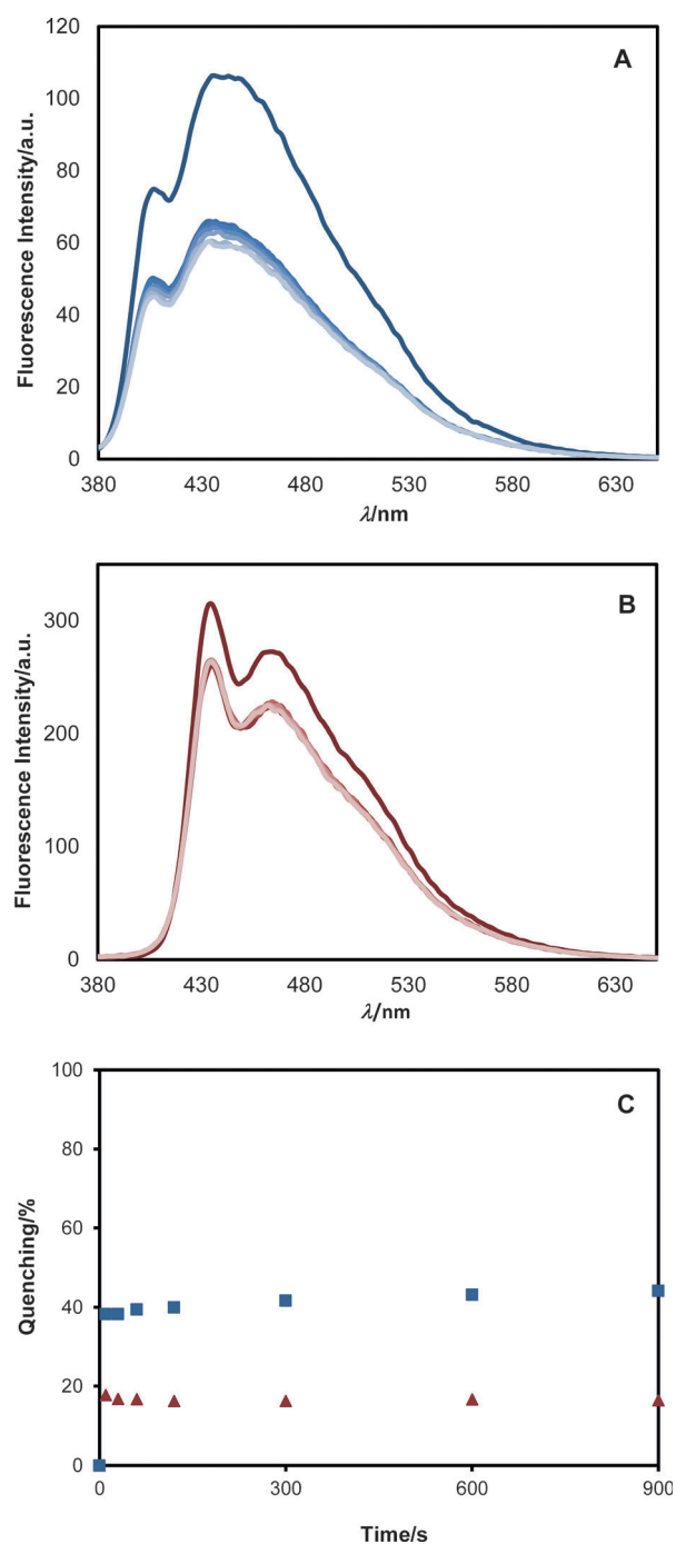
Figure 3. Time-dependent emission intensities of A) CALIX-PPE-3,6-CBZ and B) CALIX-PPE-2,7-CBZ thin films ( \approx 20 nm) after being exposed to saturated DMNB vapor (2.7 ppm) at 25 °C (0, 10, 30, 60, 90, 120, 300, 600, and 900 s, from top to bottom), and the corresponding fluorescence quenching efficiencies (C) for both materials ( \blacksquare from A, \blacktriangle from B; \lambda_{\text{exc}} = 360 nm).
