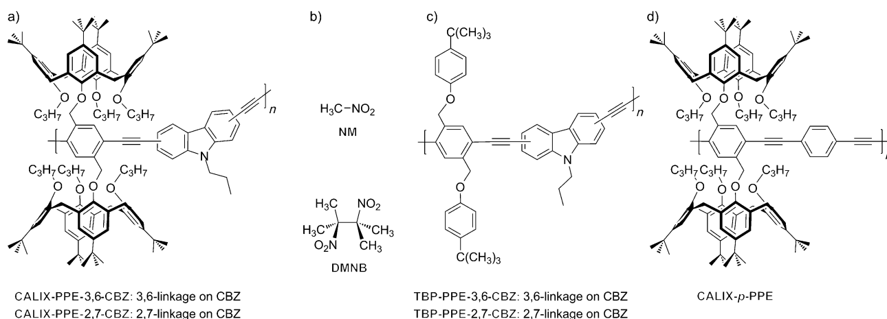
Scheme 1. Molecular structures of a) poly( \{2,5\text{-bis-[5,11,17,23-tetrakis(1,1-dimethylethyl)-25-(oxymethyl)-26,27,28-tripropoxy]calix[4]arene}\} - p -phenylene)ethynylene- alt -3,6 or 2,7-carbazolyleneethynylene (CALIX-PPE-CBZs); b) NM and DMNB; c) poly( \{2,5\text{-bis}(p\text{-tert-butylphenoxy)methyl}\} - p -phenylene)ethynylene- alt -3,6 or 2,7-carbazolyleneethynylene (TBP-PPE-CBZs); and d) poly( \{2,5\text{-bis-[5,11,17,23-tetrakis(1,1-dimethylethyl)-25-(oxymethyl)-26,27,28-tripropoxy]calix[4]arene}\} - p -phenylene)ethynylene- p -phenylene ethynylene (CALIX- p -PPE).
