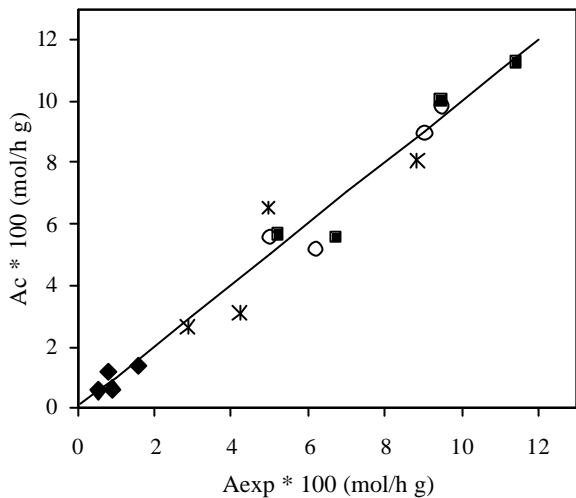
Figure 1 - Plot of the calculated, A_c , versus experimental, A_{exp} , activity values for the transformation of \blacklozenge - ethene, * - propene, \circ - 1-butene and \blacksquare - iso-butene over HNaUSY zeolites.
