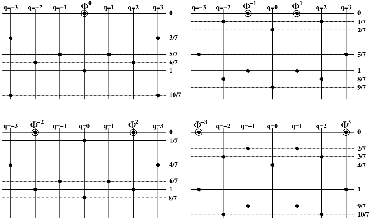
Figure 1: Representation modules for N = 7 . We show the level structure of the modules of a singlet (top left), a doublet 1 (top right), a doublet 2 (bottom left), and a doublet 3 operator (bottom right).
