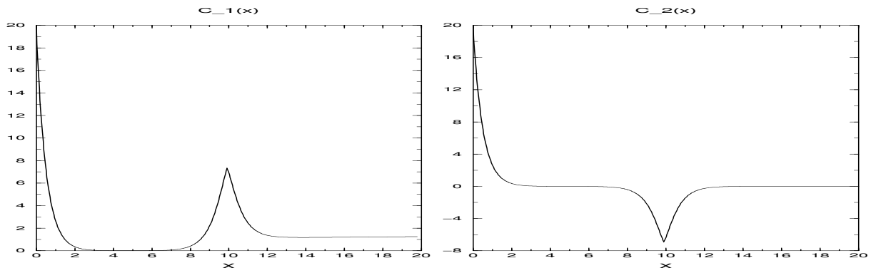
Figure 2: Two dimensional correlation function C_1(x) and C_2(x) with \nu = 10^{-4} , r_l = 1 and \rho(E) = 1 .
