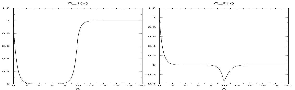
Figure 1: One dimensional correlation function C_1(x) and C_2(x) with \nu = 10^{-4} , r_l = 1 and \rho(E) = 1 .
