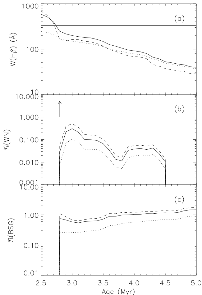
Fig. 5. Same as Fig. 4 for Z=0.008
