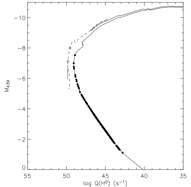
Fig. 20. (\log Q(\text{H}^0), M_{439}) diagram of the detected stars along the theoretical isochrone. The WR branch is the dashed part of the curve.
