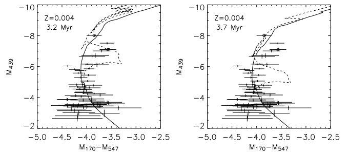
Fig. 12. Observed vs. isochrone (M_{439}, M_{170} - M_{547}) diagram for Z=0.004 . The two WR stars are marked with open circles. The WR branches of the isochrones are shown as dashed lines.
