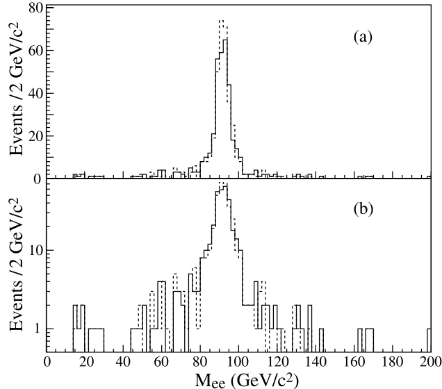
FIG. 1: Z(\rightarrow ee) + 2j data before (solid) and after (dashed) revertexing: (a) has a linear scale and illustrates the improvement in the Z -boson mass resolution after the revertexing; (b) has a logarithmic scale and shows the suppression of the background from vertex misidentification in the tails of the Z -boson peak.
