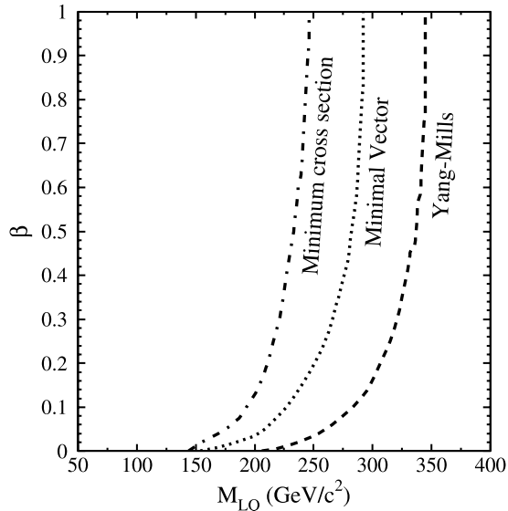
FIG. 24: The 95% C.L. lower limits on M_{LQ} as a function of \beta for first-generation vector leptoquarks with Yang-Mills, minimal vector, and minimum cross section couplings from the eejj , e\nu jj , and \nu\nu jj channels combined.
