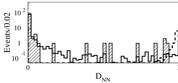
FIG. 4: Comparison of D_{NN} distributions for the predicted background (solid line histogram), 200 \text{ GeV}/c^2 leptoquark events (dashed line histogram), and the data (hatched histogram).
