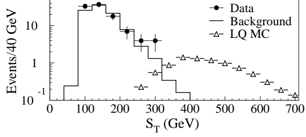
FIG. 2: S_T distributions for background (solid line histogram), data (solid circles), and M_{LQ} = 200 \text{ GeV}/c^2 MC events (open triangles) for the eejj analysis.
