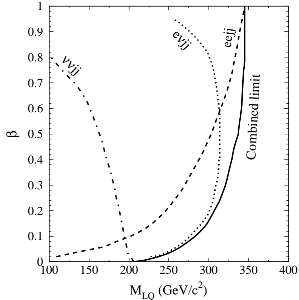
FIG. 23: The 95% C.L. lower limit, as a function of \beta , on the mass of first-generation vector leptoquarks with Yang-Mills couplings from the individual eejj , e\nu jj , and \nu\nu jj channels and for the combined analysis.
