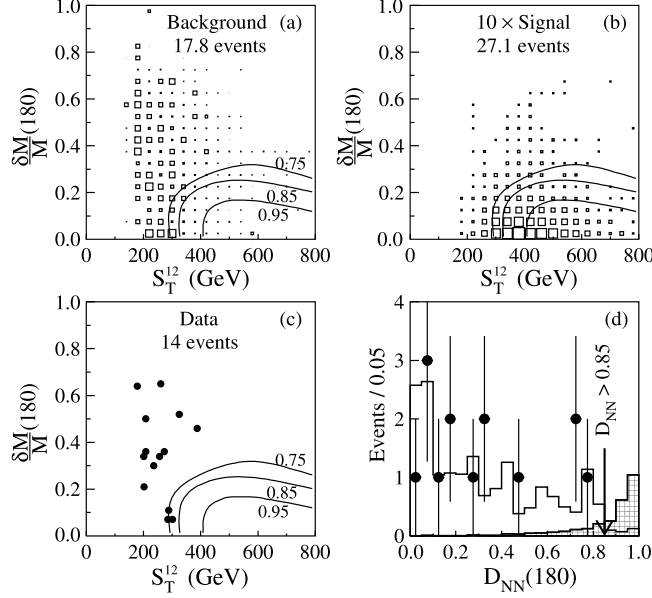
FIG. 16: Distributions of \frac{\delta M}{M}(180) versus S_T^{12} for (a) the total background, (b) ten times the expected signal from 180 GeV/ c^2 leptoquarks, and (c) the data. (d) The neural network discriminant for the signal (hatched histogram), the background (open histogram), and the data (points with error bars). The curves show neural net contours for D_{NN} = 0.95, 0.85, and 0.75 .
