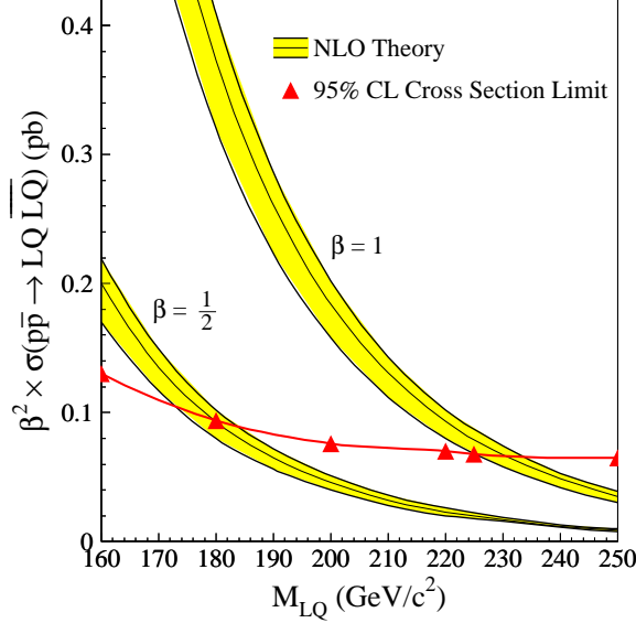
FIG. 10: Upper limit on the leptoquark pair-production cross section (triangles) from the eejj channel. The NLO calculations of Ref. [22] for \beta = 1 (upper band) and \beta = \frac{1}{2} (lower band) are also shown. The central lines correspond to \mu = M_{\text{LQ}} , and the lower and upper edges of the bands correspond to \mu = 2M_{\text{LQ}} and \mu = \frac{1}{2}M_{\text{LQ}} , respectively.
