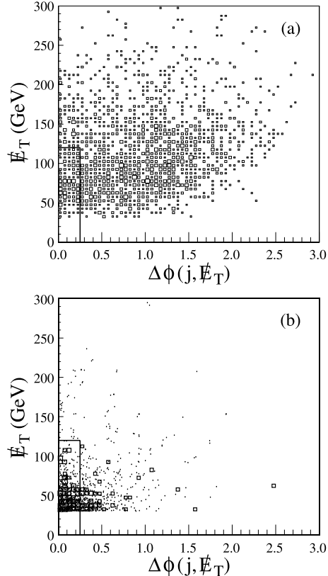
FIG. 13: Effect of the requirement of acolinearity in \cancel{E}_T on (a) a 180 \text{ GeV}/c^2 MC leptiquark signal and (b) the multijet background. In (b), the dots show the distribution before imposition of the M_T^{e\nu} requirement; the open squares show the distribution after applying the M_T^{e\nu} requirement. The acolinearity requirement is indicated by the solid lines.
