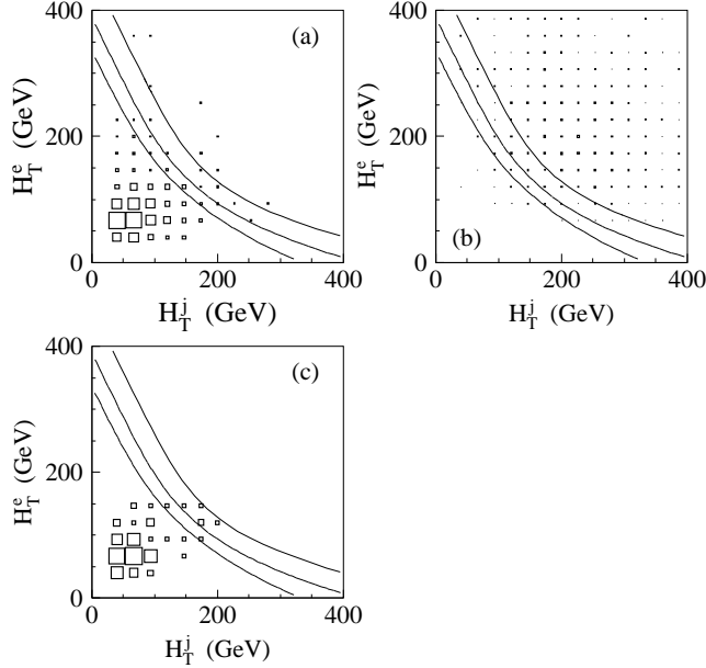
FIG. 5: H_T^e versus H_T^j for (a) the predicted background, (b) 200 \text{GeV}/c^2 leptoquark events, and (c) the base data sample. The curved lines correspond to \mathcal{D}_{\text{NN}} = 0.5, 0.8, and 0.95 (from left to right). The area of a displayed square is proportional to the number of events in that bin, with the total number of events normalized to 123 \text{ pb}^{-1} .
