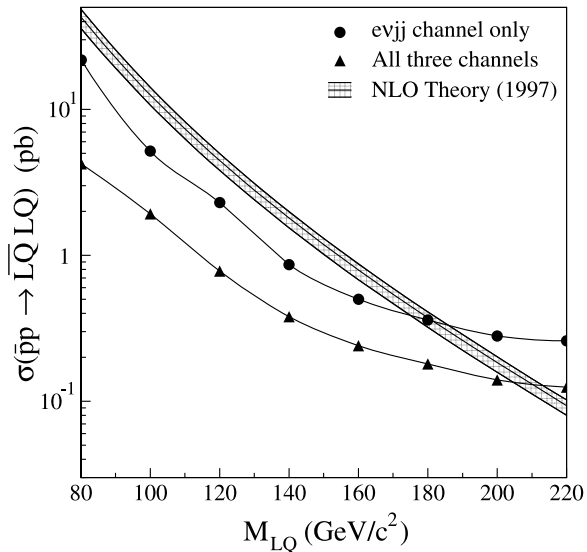
FIG. 18: The 95% C.L. upper limits on the cross sections for scalar leptoquark pair production from the evjj channel, and for all three channels combined, for \beta = \frac{1}{2} , compared to the NLO prediction, as a function of leptoquark mass.
