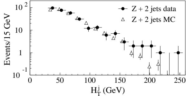
FIG. 6: The H_T^j distribution for Z + 2j data (solid circles) and MC (open triangles) in the Z boson mass region. For high-mass DY events, S_T \approx 350 GeV corresponds to H_T^j \approx 100 GeV.
