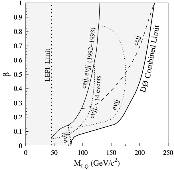
FIG. 22: The 95% C.L. lower limit on the mass of first-generation scalar leptoquarks as a function of \beta for the individual eejj , evjj , and \nu\nu jj channels, and for the combined analysis.
