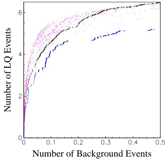
FIG. 3: Predicted number of M_{LQ} = 200 \text{ GeV}/c^2 events versus the predicted number of background events for three RGSEARCH runs. The upper dotted line shows the variation with S_T . The lower dotted line shows the variation with \frac{\delta M}{M}(200) . The structure (gaps) arises from an increase in acceptance for DY events. The more dispersed set of dots shows the result when both S_T and \frac{\delta M}{M}(200) are varied. The density of points is irrelevant.
