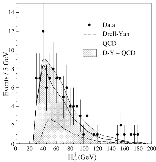
FIG. 7: Fit of the H_T^j distribution in the eejj data to the sum of the DY and multijet backgrounds.
