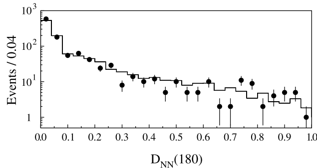
FIG. 17: Comparison of the D_{NN}(180) distribution for the e\nu jj data (points with error bars) and the predicted background (solid histogram) before the cut on M_T^{e\nu} .
