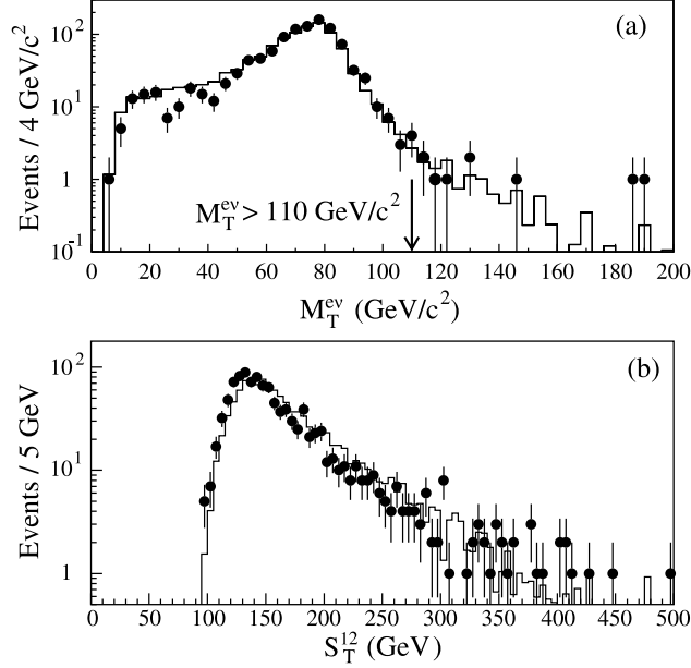
FIG. 14: Comparison of the (a) M_T^{e\nu} and (b) S_T^{12} distributions for the e\nu jj data (points with error bars) and the predicted background (solid histogram) before imposing the M_T^{e\nu} requirement.
