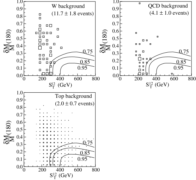
FIG. 15: Distributions of \frac{\delta M}{M}(180) versus S_T^{12} for the three individual backgrounds: (a) W + 2j events, (b) multijet events, and (c) t\bar{t} events. The curves show neural net contours for \mathcal{D}_{NN}(180) = 0.75, 0.85, and 0.95 .
