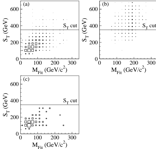
FIG. 8: S_T versus the fitted mass for (a) background, (b) 200 \text{ GeV}/c^2 leptoquarks, and (c) the base data sample. The area of a displayed square is proportional to the number of events in the bin.
