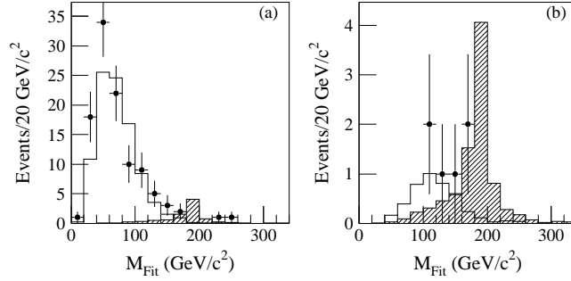
FIG. 9: Distributions of fitted mass for the events in the base data sample (solid circles), expected background (solid line histogram), and 200 \text{ GeV}/c^2 leptiquarks (hatched histogram) with (a) no cut on S_T and (b) a reduced threshold of S_T > 250 \text{ GeV} .
