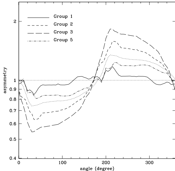
Figure 26. The asymmetry signal as a function of position angle for the variable stars in groups 1, 2, 3 and 5. The dotted curve shows the asymmetry signal of the 35414 variable stars in the catalogue. Both Fig. 26 and Fig. 27 are not corrected for the effects of M32 or HD 3914, but we have shown in the text that the correction is small.
