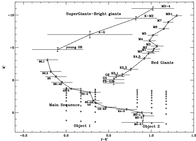
Figure 3. J - K' , M_{K'} , absolute CMD diagram computed for template main sequence stars (Ruelas-Mayorga 1991). The range of locations for the XTE J1908+094 companion star in the diagram has been derived from the absolute magnitudes of the two possible counterparts, computed taking the minimum apparent magnitudes on 2002 August 18th, and assuming that all the flux is produced from the companion star. Three different values of the interstellar extinction have been applied i.e. A_V = 11.19, 12.9, 13.9 magnitudes from right to left, respectively. A_V = 12.9 magnitudes corresponds to a column density N_H = 2.3 \times 10^{22} (Woods et al. 2002), using the relation from Predehl & Schmitt (1995). From bottom to top the crosses correspond to a source distance increasing from 1 to 10 kpc. According to the diagram, in the case of object 1, the companion star would be an intermediate/late type main sequence star of spectral type between A and K, located between 3 and 10 kpc. In the case of object 2, the companion star would be a late-type main sequence star of spectral type later than K, located between 1 and 3 kpc.
