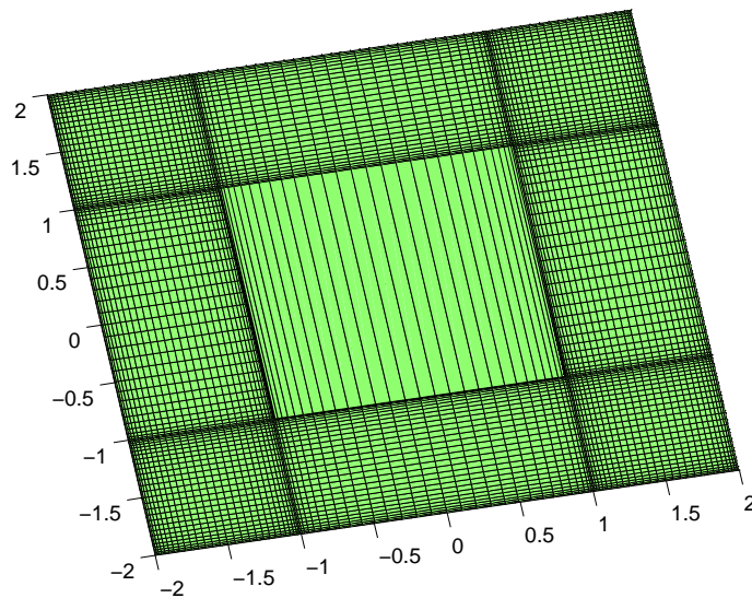
Figure 4: The square ring domain and its decomposition
