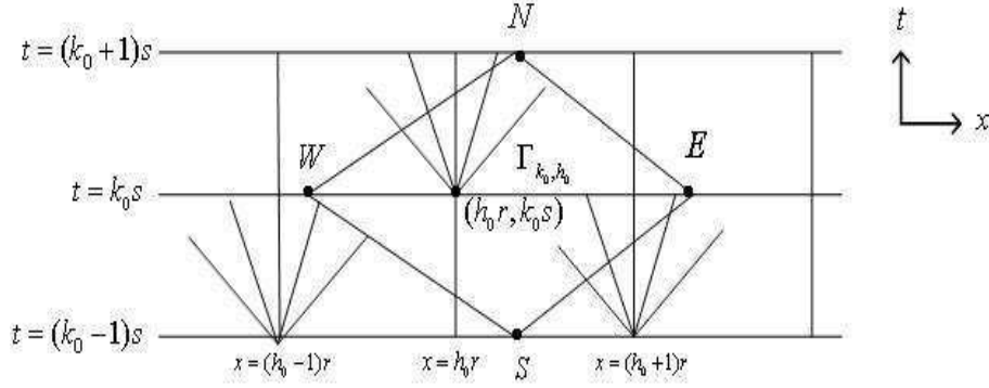
Figure 4.1 : Diamond region \Gamma_{k_0, h_0}
