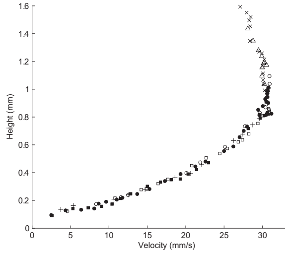
Fig. 3 Near-wall velocity profile of the density current, measured 0.3m downslope of the entrance with PST. Each symbol correspond to a different particle. \rho = 1025Kg.m^{-3} , Q = 0.95mL.s^{-1} , \theta = 16^\circ .
