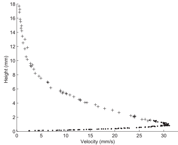
Fig. 4 Complete velocity profile. PST data from figure 3 (dots) are completed using classical side-view particle tracking (crosses).
