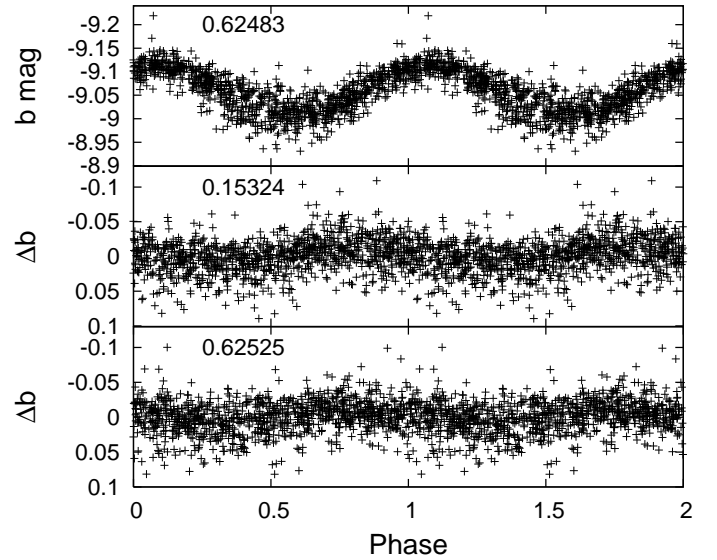
Fig. 20. Be SMC5_82941 folded in phase: top with f_1=0.62483\text{c d}^{-1} , middle with f_3=0.15324\text{c d}^{-1} after prewhitening for f_1 , and bottom with f_2=0.62525\text{c d}^{-1} after prewhitening for f_1 and f_2 .
