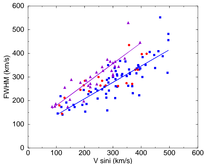
Fig. 3. FWHM of the H\alpha emission line as a function of V\sin i for Be stars with symmetric H\alpha profiles and EW\alpha > 20 \text{ \AA} . Squares correspond to Be stars in the SMC, circles to Be stars in the LMC from Paper I, and triangles to Be stars in the MW from Dachs et al. (1992), Andrillat & Fehrenbach (1982) and Andrillat (1983). The linear regression for samples in the SMC and MW is shown.
