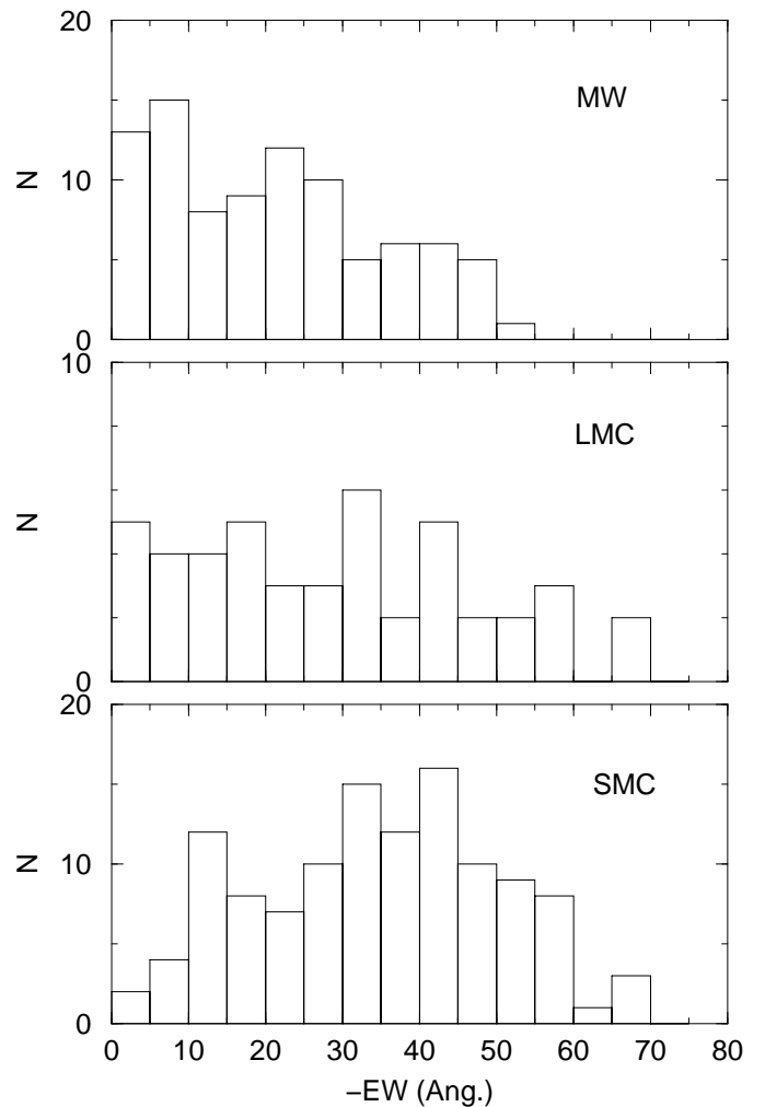
Fig. 2. Distributions of Be stars versus the EW of the H\alpha emission line. Top: in the MW from Dachs et al. (1992), Andriolat & Fehrenbach (1982) and Andriolat (1983); middle: in the LMC from Paper I; bottom: in the SMC (this study).
