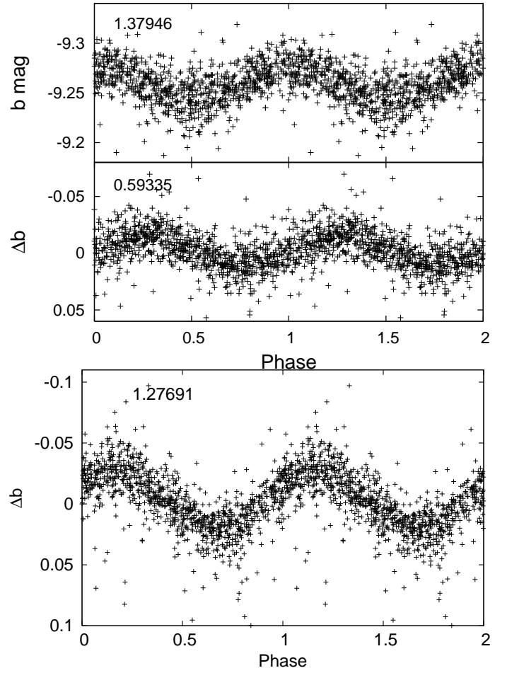
Fig. 14. Be SMC5_13978 folded in phase: top with f_1=1.37946\text{c d}^{-1} , middle with f_2=0.59335\text{c d}^{-1} after prewhitening for f_1 . Bottom: Be SMC5_14212 folded in phase with f=1.27691\text{c d}^{-1} .
