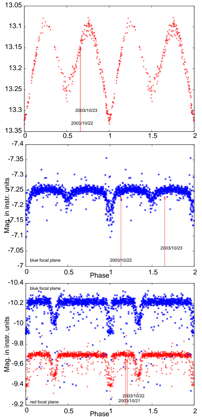
Fig. 6. Top: SMC5_002807 folded in phase with P=454.959d (OGLE data, I_{mag} ). Middle: SMC5_003789 Be star folded in phase with P=2.087d (MACHO data). Bottom: SMC5_0004477 folded in phase with P=4.480d (MACHO data).
