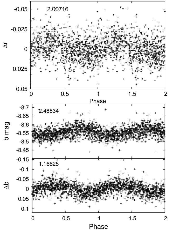
Fig. 19. Top: Be SMC5_43413 folded in phase with f=2.00716\text{c d}^{-1} . Be SMC5_82042 folded in phase: middle with f_1=2.48834\text{c d}^{-1} , bottom with f_2=1.16625\text{c d}^{-1} after prewhitening for f_1 .
