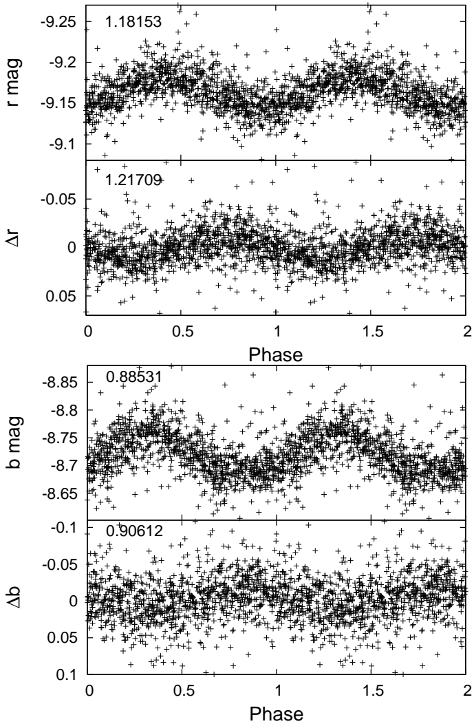
Fig. 18. Be SMC5_37013 folded in phase: top with f_1=1.18153\text{c d}^{-1} , middle up with f_2=1.21709\text{c d}^{-1} after prewhitening for f_1 . Be SMC5_37162 folded in phase: middle down with f_1=0.88531\text{c d}^{-1} , bottom with f_2=0.90612\text{c d}^{-1} after prewhitening for f_1 .
