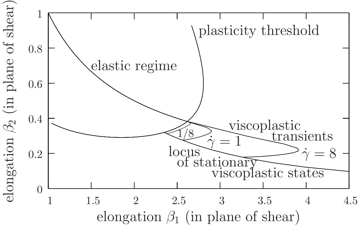
FIG. 18: Form of the stored elastic deformation in the course of an experiment and in the stationary regime, for three different values of the shear rate \dot{\gamma} . The axes are the first two eigenvalues, \beta_1 and \beta_2 , of tensor B .
