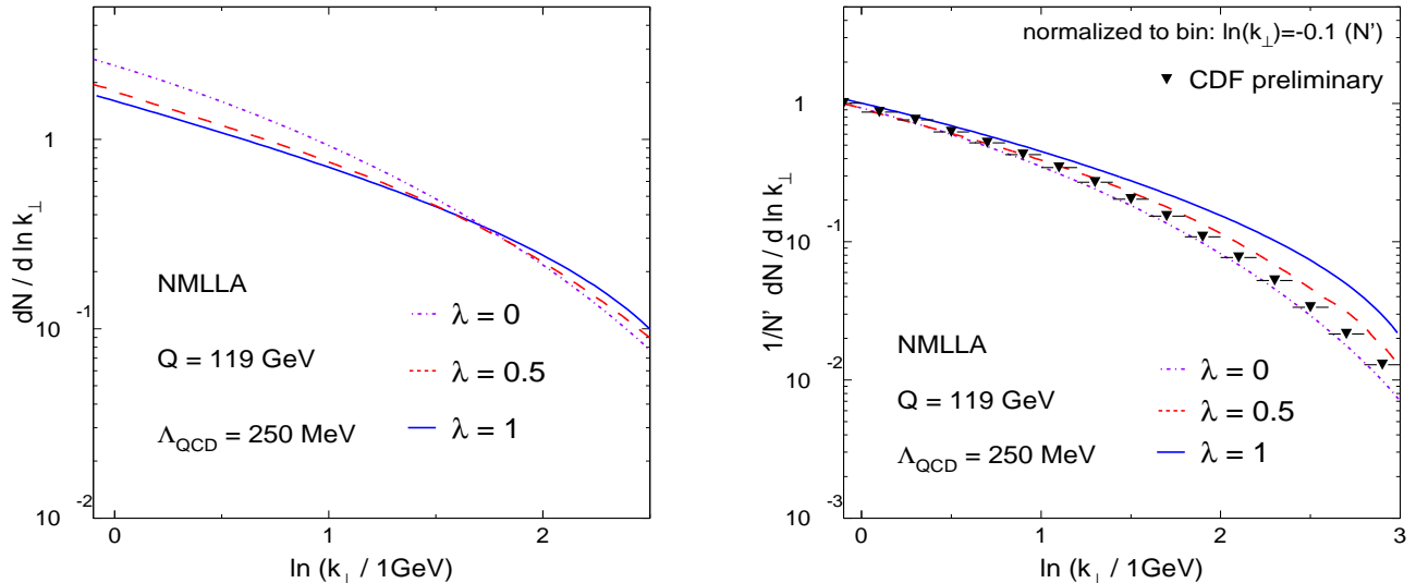
Figure 10: Absolute (left) and normalized (right) inclusive k_{\perp} -distribution beyond the limiting spectrum approximation at NMLLA in a jet of hardness Q = 119 GeV.
